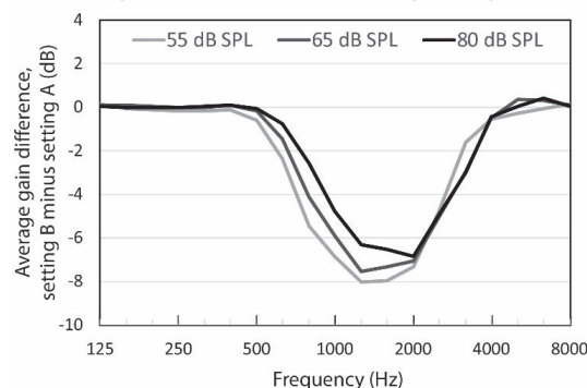
Figure 1. Long-term average gain difference between settings B and A, averaged across all participants. Gain measurements made using a speech signal at three input levels, 55, 65, and 80 dB SPL.
