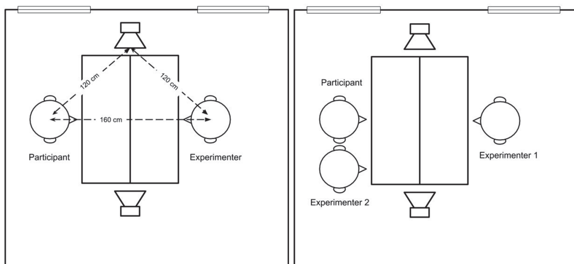
Figure 2. LEAP test setups. The left panel shows the setup for test scenario 1 and 2 (Conversation 2 people). The right panel shows the setup for test scenario 3 (Conversation 3 people).
