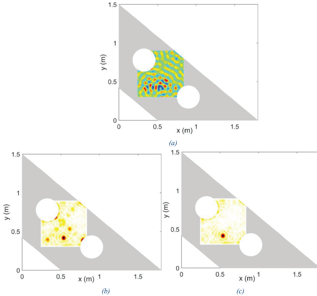
Figure 3: (a) displacement field (m) measured (numerical experiment) on the real structure in the zone of the virtual structure at 2100Hz; (b) force distribution ( \text{N/m}^2 ) identified using the virtual structure without stiffeners (Figure 2 (b)); (c) force distribution identified using the virtual structure with stiffeners (Figure 2 (c))
