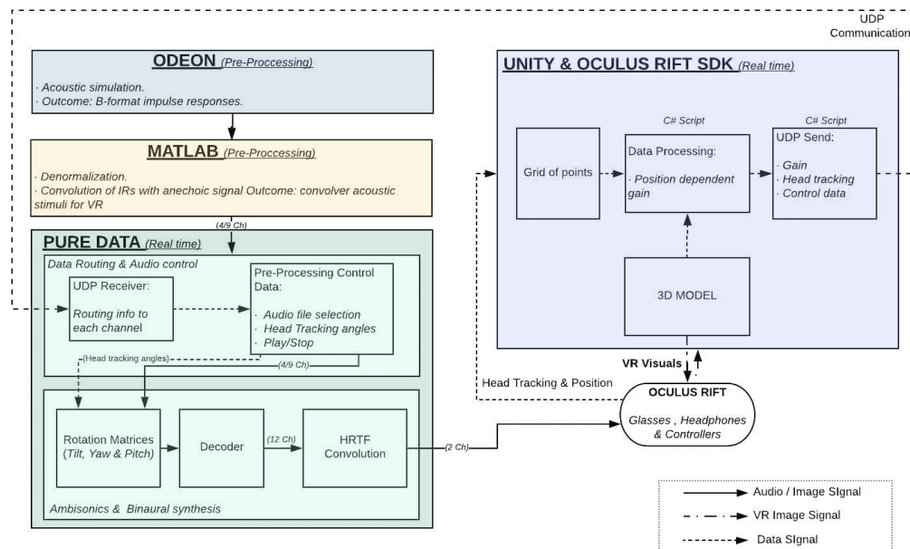
Figure 1. Flow chart illustrating the AVR system.
