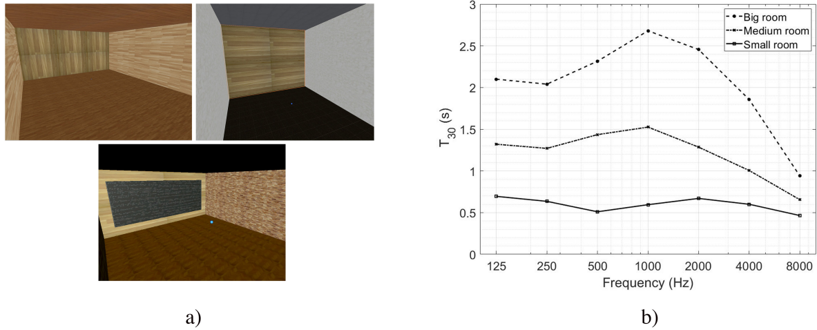
Figure 3. a) A screen capture from Unity showing the big room (top left), medium room (top right) and small room (bottom). The listening position is shown as a blue sphere. b) Simulated reverberation times for the three room types used in the localization experiment.
