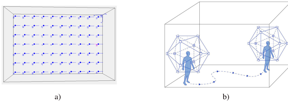
Figure 2. a) An example of a receiver grid in a simple room in Odeon. b) Illustration of the icosahedron loudspeaker array used in the AVR implementation and how it follows the listener in the virtual space.
