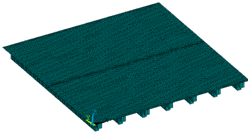
Figure 3. FE model of the assembled floor in ANSYS.
