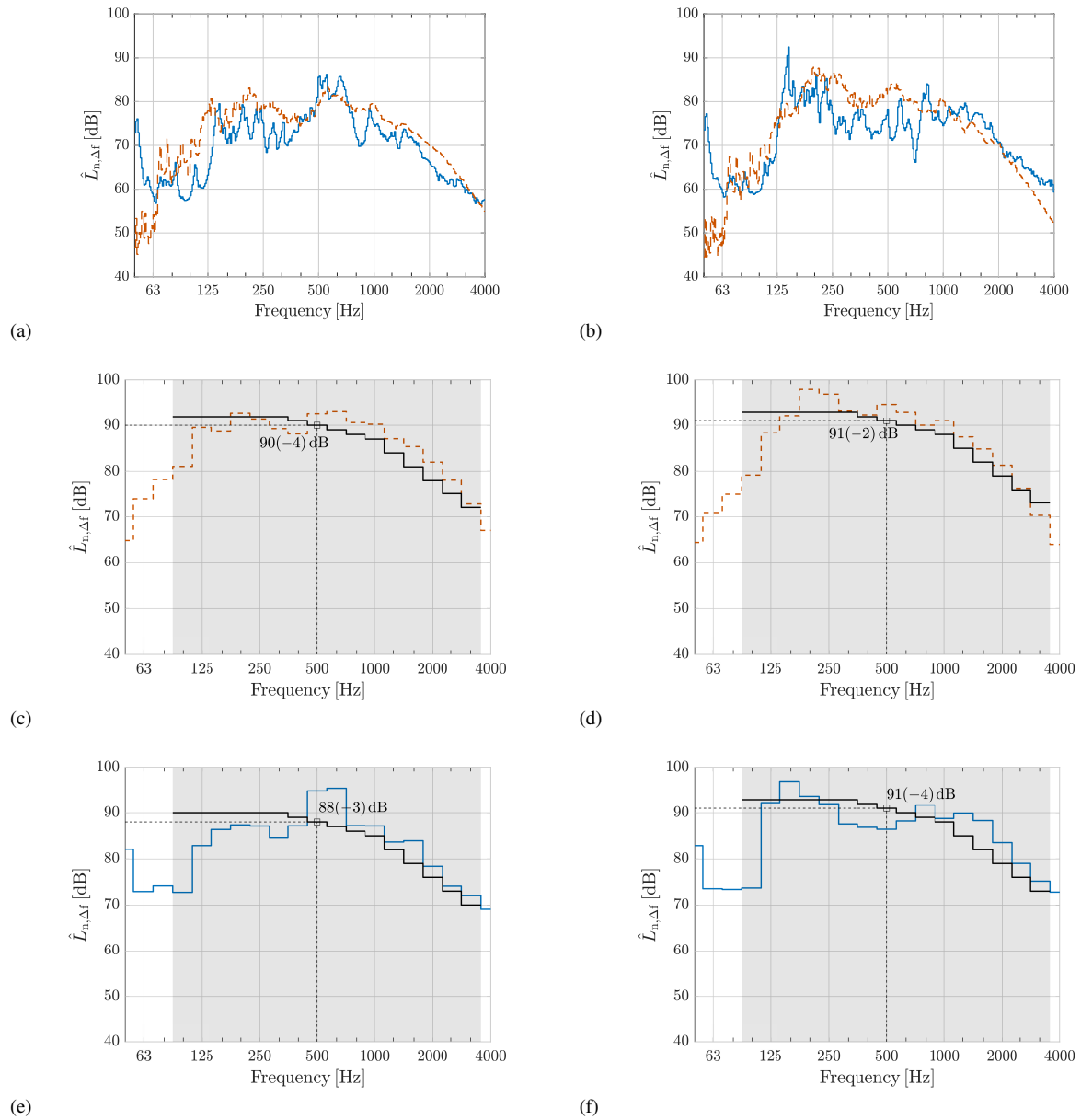
Figure 5. Measured (red dashed line) and computed (blue solid line) normalized sound pressure levels in the receiving room integrated over (a,b) 1/48-octave bands and (c-f) 1/3-octave bands, and averaged over tapping machine excitations at (a,c,e) eight beam positions and (b,d,f) eight inter-beam positions of the floor. The measured results are also averaged over the microphone positions in the room. Plots (c-f) additionally display shifted reference curves (black) and single number rating values L_{n,w}(C_1) in accordance with ISO-717-2-1996. The gray zones indicate the frequency range for single number ratings.
