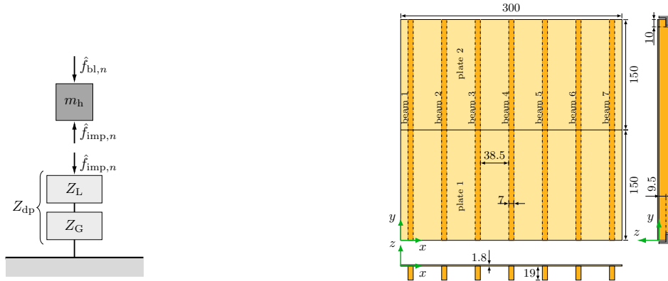
Figure 1. Model for the ISO tapping machine hammer excitation on a floor.
