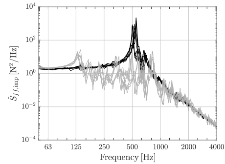
Figure 4. Computed power spectra densities of squared impact force spectra of excitations on eight beam positions (black solid line) and eight inter-beam positions (gray solid line) in the sound radiation test.
