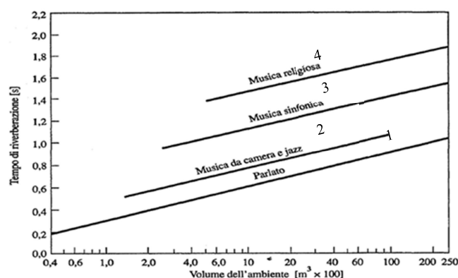
Figure 9: RT Trend related to the use destination of the volume (1 speech, 2 jazz and chamber music, 3 symphonic music, 4 religious music)
