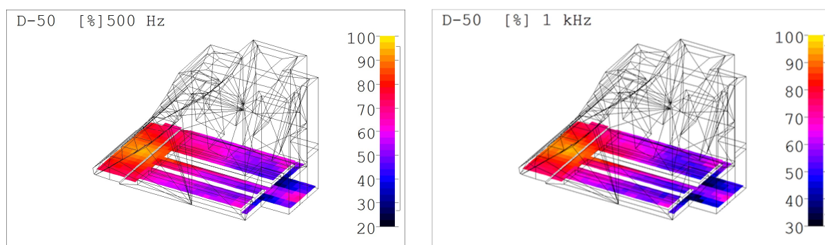
Figure 5 and 6: 3D model SRC 1 - Definition ( D_{50} ) at 500 Hz and 1kHz
