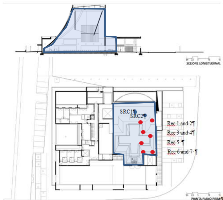
Figure 1 and 2. The church longitudinal section and plan (source position are colored blue, receivers are colored red)
