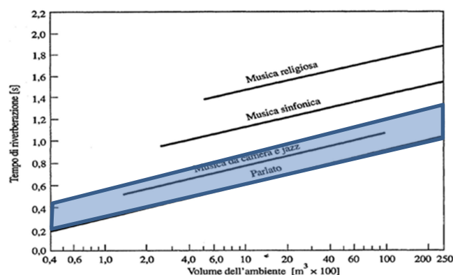
Figure 10: Trend Area for contemporary churches RT colored in blue
