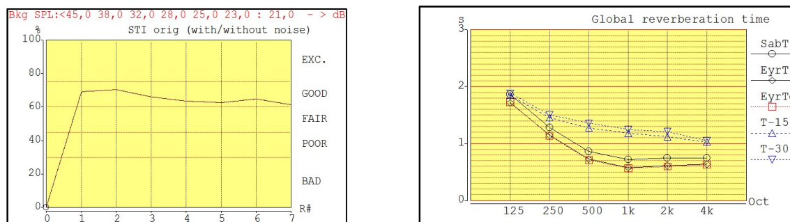
Figure 7 and 8: STI Values and Trend and RT Sabine (SabT), RT Eyring (EyrT), T_{30} and T_{15}
