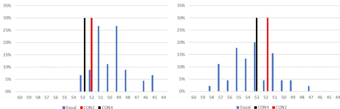
Figure 5 Left - Distribution of answers for pair CON2 – CON4 compared with calculated values of L_{n,w}+C_{l,50-2500} , Right - example of CON4 – CON2
