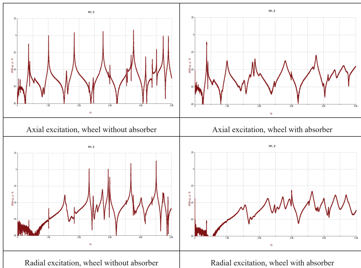
Figure 4 – Transfer functions of the BVV-5L wheel measured with impact hammer and acceleration sensor.
