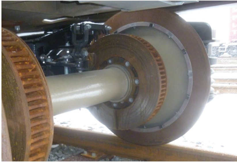
Figure 1 – This is a BVV-wheelset with wheel absorber in a vehicle of the 5L project
