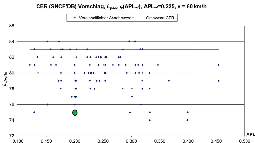
Figure 5 – Overview of TSI levels from the UBA report (8) supplemented by one point for the level of the 5L project (75 dB / APL 0.2).
