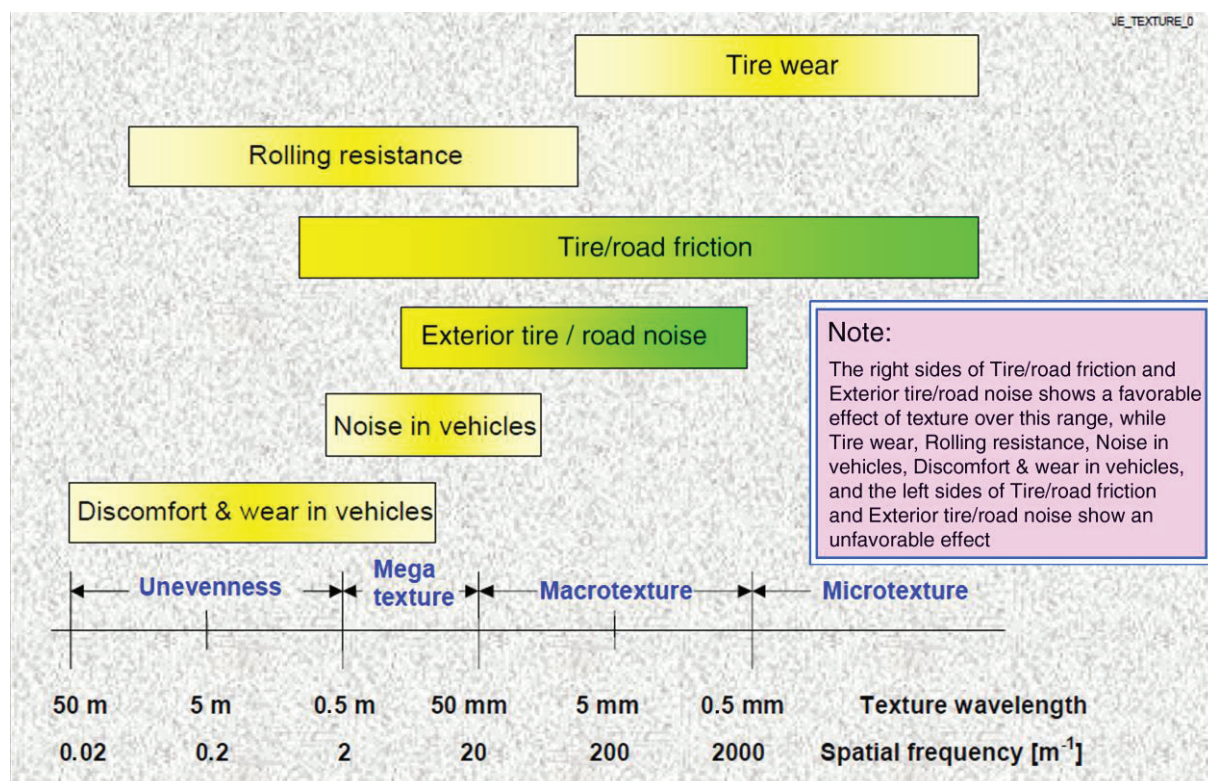
Figure 1 Illustration of texture wavelengths, anticipated effects showing that noise is affected by macrotexture (4)
