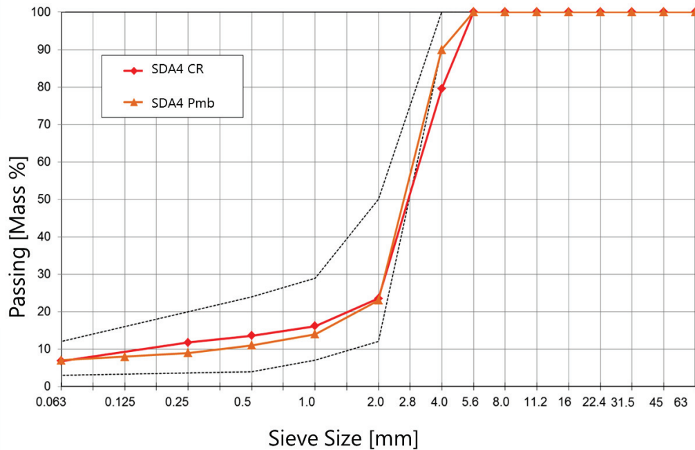
Figure 2 Aggregate size distribution of SDA-4 with polymer modified bitumen and with straight run bitumen 50/70 and 1% CR
