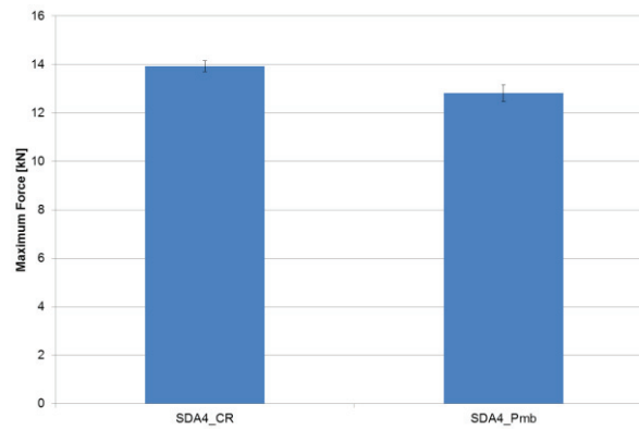
Figure 5 Maximum force to mechanical failure as a result of the indirect tensile tests
