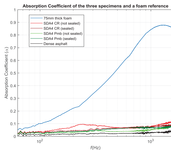
Figure 7 Absorption coefficient of the three asphalt samples in comparison to a highly absorbent foam sample
