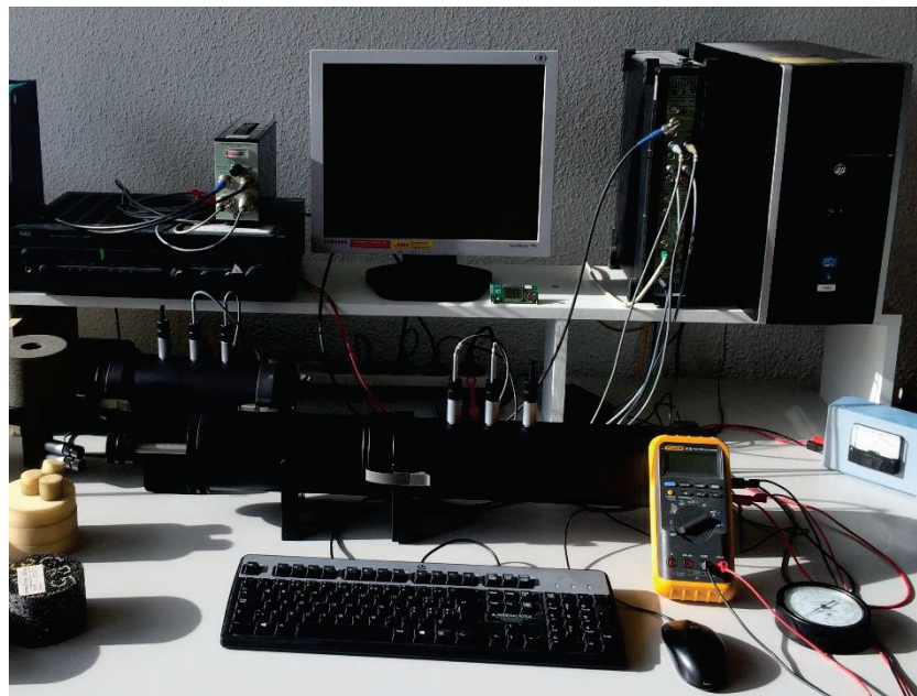
Figure 4 Acoustic test setup showing the impedance tube and data acquisition devices
