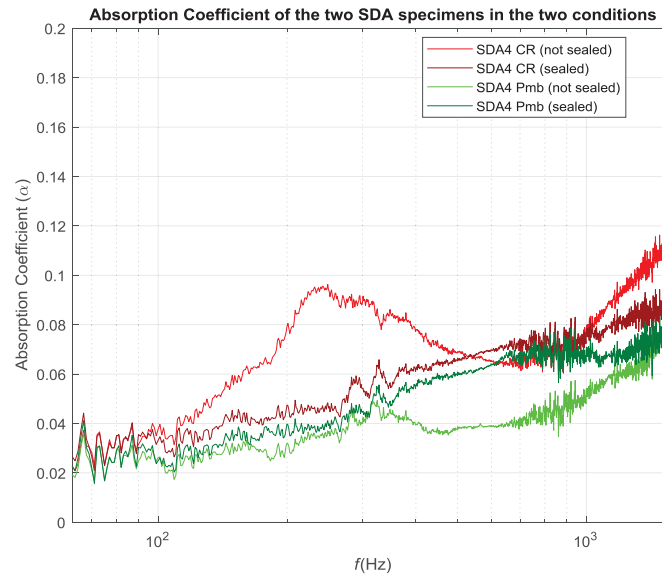
Figure 6 Absorption coefficient of two SDA specimens in two conditions
