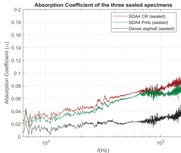
Figure 8 Absorption coefficient of SDA4_CR; SDA4_Pmb and dense asphalt
