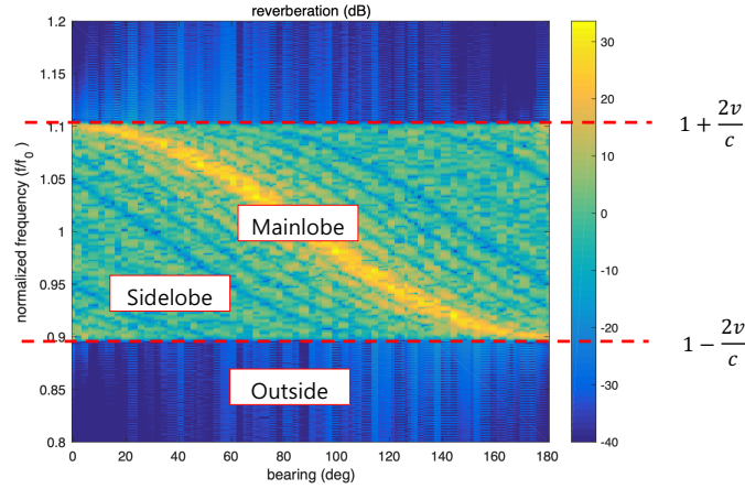
Figure 1. Simulated reverberation of a frequency-bearing domain. The receiver is assumed to use beamformers. The x-axis denotes a bearing and the y-axis denotes a relative frequency.
