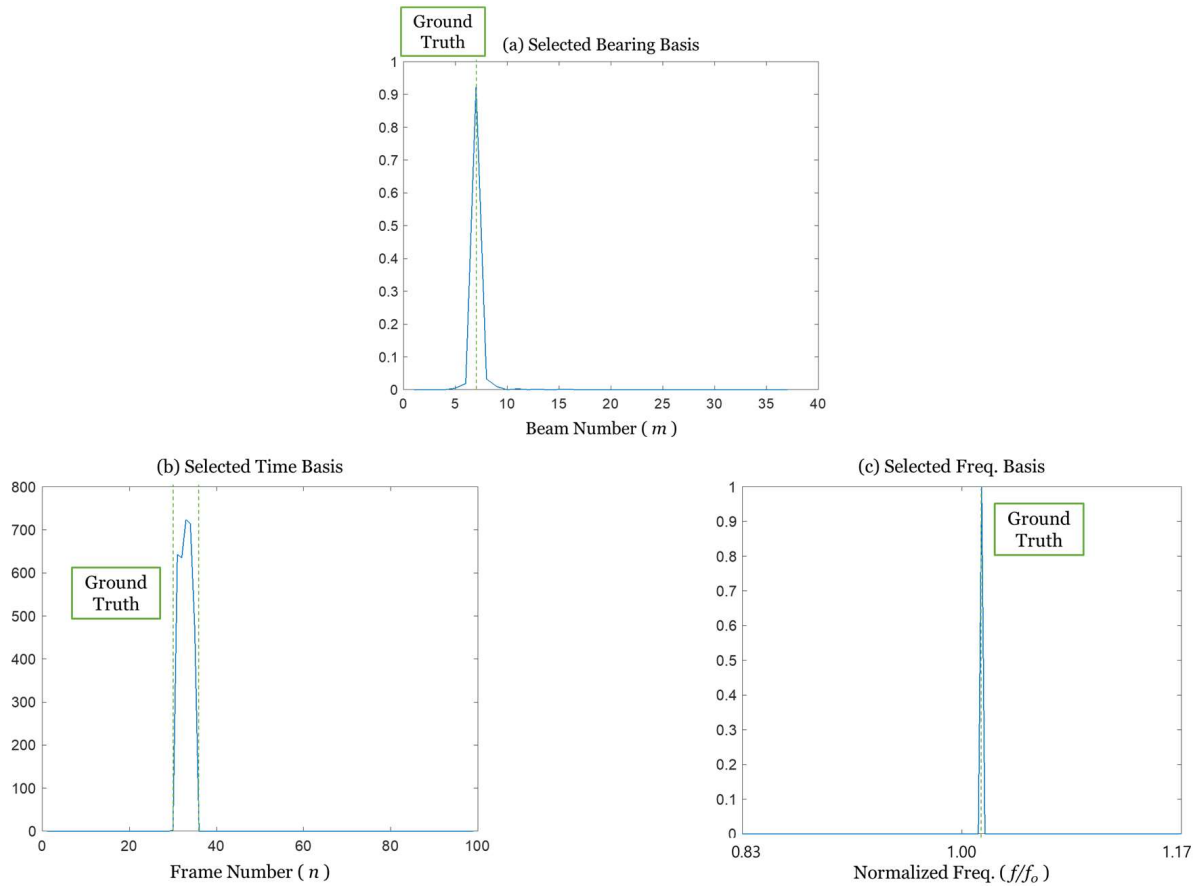
Figure 4. Selected (a) bearing, (b) time, and (c) frequency basis vectors. Green dashed line denotes the ground truth.
