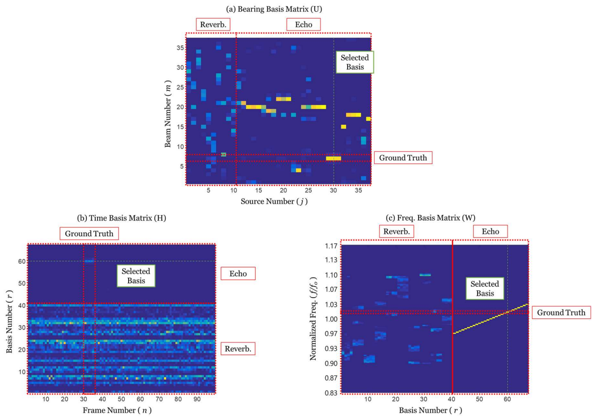
Figure 3. Results of estimated (a) bearing, (b) time, and (c) frequency basis matrices. Red dotted rectangles denotes the reverberation and echo basis groups, and the ground truth to be estimated. Green dashed line denotes the selected basis r_{target} by the proposed algorithm.
