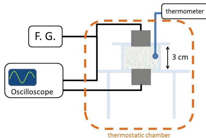
Figure 1 – A diagram of sediment sound speed measuring system.
