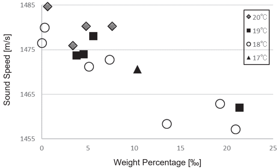
Figure 2 – Estimated sound speed according to the weight percentage.
