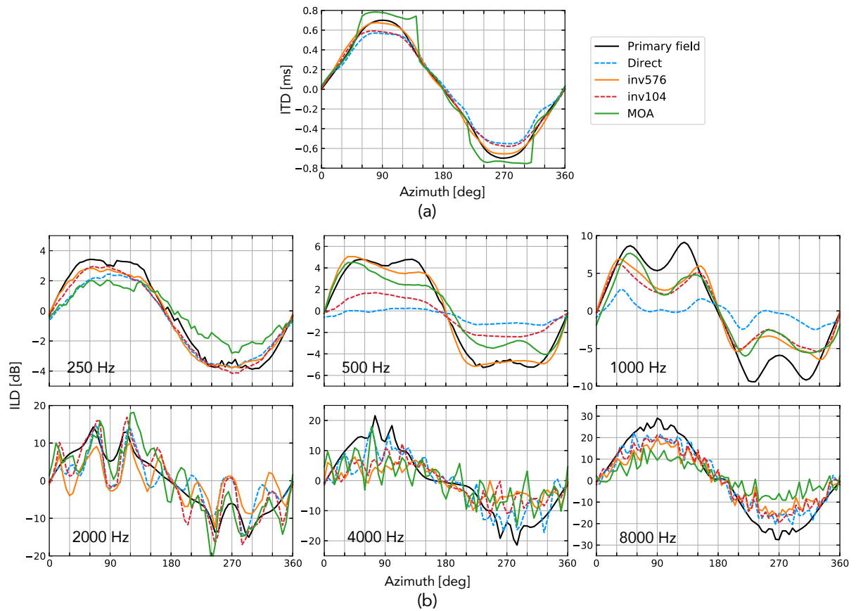
Figure 4. Interaural time and level difference; (a) Interaural time difference in primary and reproduced field which calculated using the cross-correlation function for the left and right of the dummy head signals passed through the 1600 Hz LPF. (b) Interaural level difference in primary and reproduced field calculated every 250 Hz to 8,000 Hz 1/1 octave bands.
