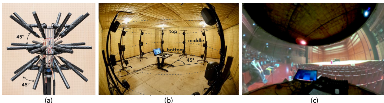
Figure 1. Systems overview; (a) the Hedgehog microphone array which consists of 24 narrow directional microphones, (b) the loudspeaker array of stacked-ring layout in three layers, and (c) image when presenting sound and video using a cylindrical screen installed inside the loudspeaker array.
