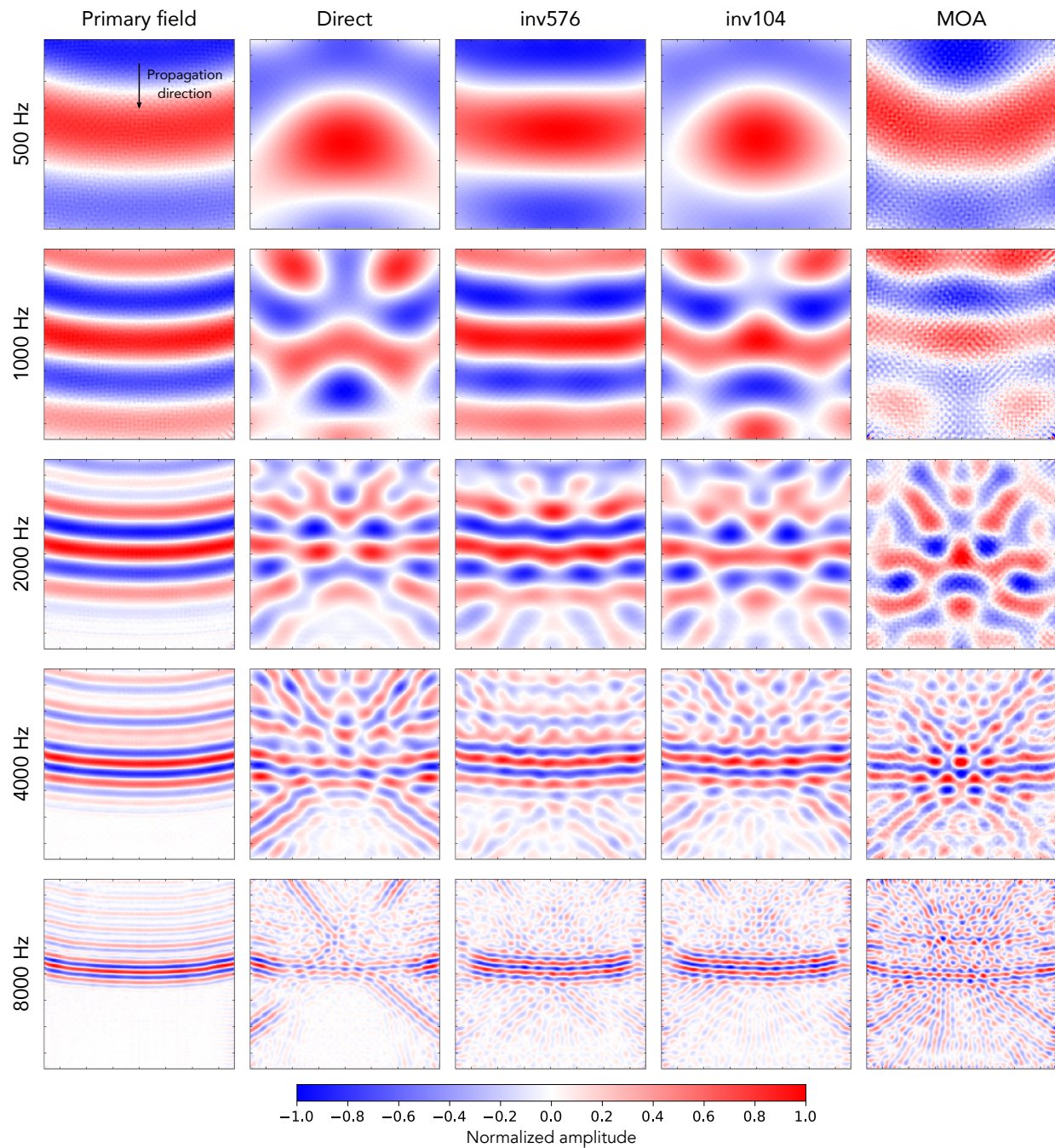
Figure 3. Horizontal wavefront measured in the primary field and the reproduced field with Direct, inv576, inv104, and MOA. The sound source was an impulse passed through one-octave bandpass filter emitted from a loudspeaker placed 2 m away from the center of the visualization area. The frequency described on the left side represents the center frequency of the bandpass filter.
