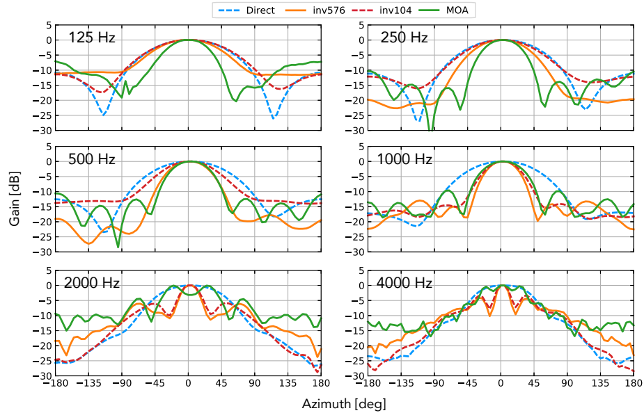
Figure 2. Equivalent directivity obtained by measuring the speaker output levels while rotating the Hedgehog array in the primary field
