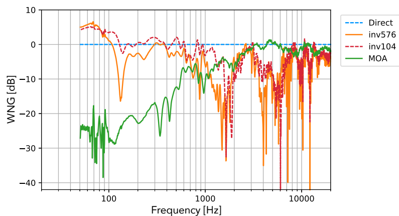
Figure 5. Measured white noise gain for the front loudspeaker signal in the case where the sound source of the primary field is also in the front direction. A positive WNG indicates an improvement in SNR.
