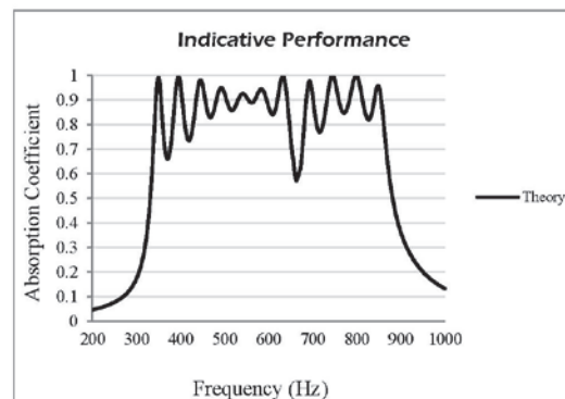
Figure 13 – indicative design
