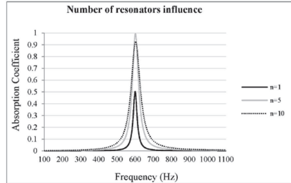
Figure 7 – number of resonators influence
