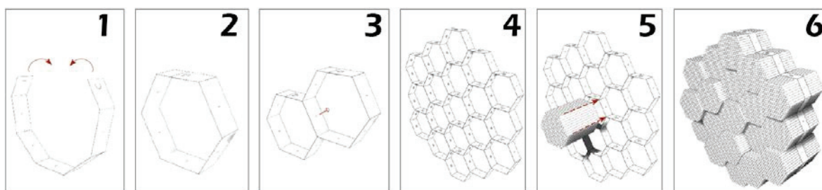
Figure 15 – assembly steps
