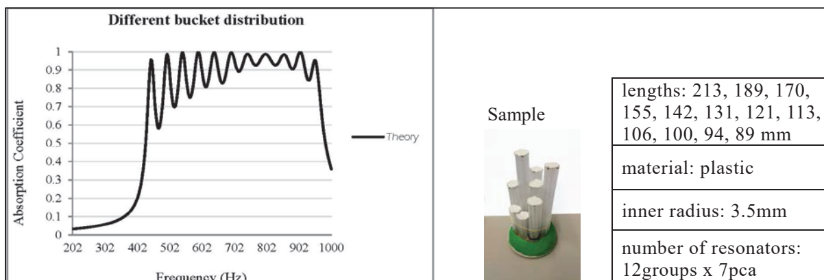
Figure 5 – broadband absorption
