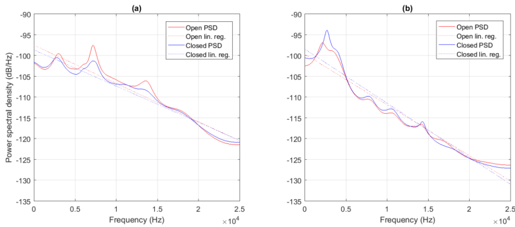
Figure 8 – Power spectral density (PSD) of the noise with respect to voice quality and glottal phase, and linear regression models of the PSDs. (a) Breathy voice quality, and (b) Normal voice quality.
