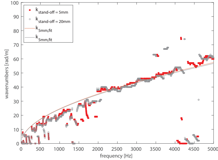
Figure 3. Comparison between the wavenumber dispersion relations determined by using the wave correlation approach from sound pressure measurements performed at 20 mm and at 5 mm from the panel surface.
