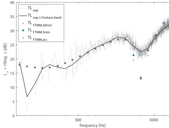
Figure 4. Comparison between the experimental transmission loss of the plywood panel and the numerical results calculated using as input data the elastic properties presented in Table 1
