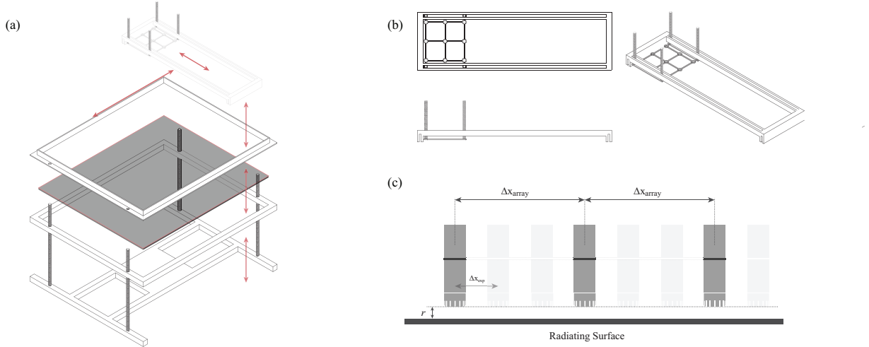
Figure 1. Test rig for the mechanical characterisation of lightweight panels: (a) exploded diagram of the testing frame and the scanning microphone carriage; (b) views of the scanning microphone carriage; (c) diagram of the sound pressure scanning system.
