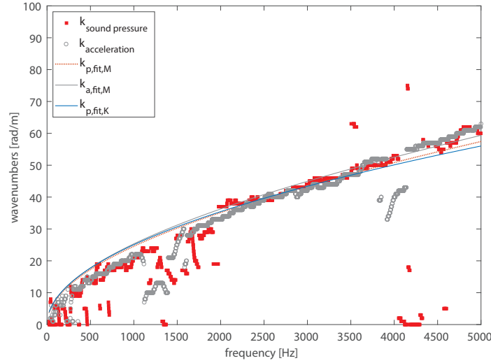
Figure 2. Comparison between the experimental wavenumber dispersion relation determined by using the wave correlation approach from sound pressure measurement k_p and acceleration measurements k_a , and between the curves obtained by analytical fitting k_{i,fit,j} .
