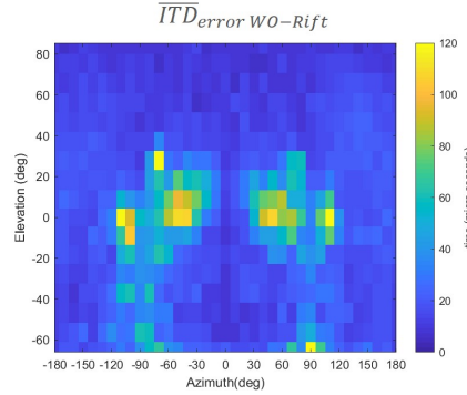
Figure 5. \overline{ITD}_{error} averaged for all subjects and KEMAR
