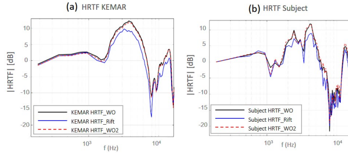
Figure 1. HRTF magnitude over the front direction for (a)KEMAR and (b)human subject for the left ear.
