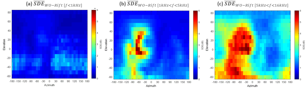
Figure 3. \overline{SDE}_{WO-Rift}(\Omega) averaged across all subjects and KEMAR for three different frequency bands (a) low frequency, (b) mid frequency and (c) high frequency.
