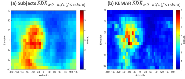
Figure 2. \overline{SDE}_{WO-Rift}(\Omega) averaged across frequency for (a) all human subjects and (b) KEMAR manikin.
