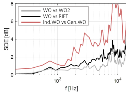
Figure 4. SDE averaged across all direction for one subject. SDE was calculated for three pairs of HRTFs
