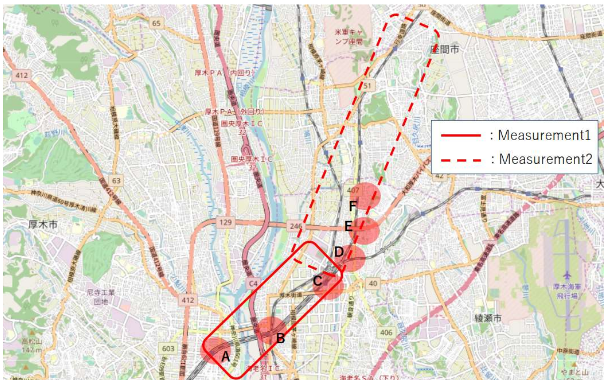
Fig.1—Target section in survey 1 and 2 (Hon-Atsugi – Sagami-ono Stations up and down lines) * A to F in the figure indicate curved trajectories. © CCBYSA / OpenStreetMap contributors
