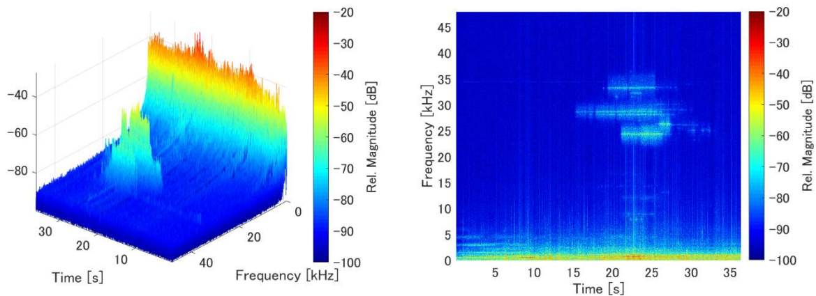
Fig. 3— FFT analysis result of survey 1 (B: Atsugi ~ Ebina).
