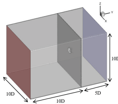
Figure 3 – Computational domain for virtual fan performance tester
