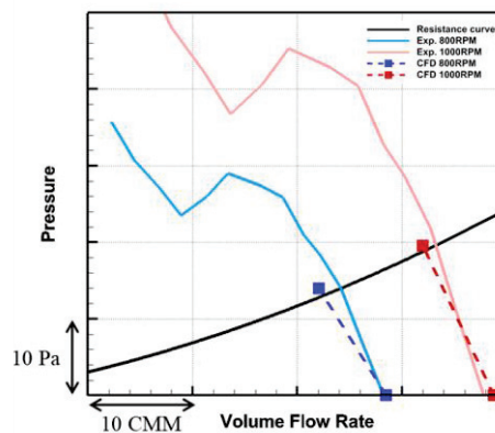
Figure 4 – Comparison of predicted volume flow rate at a given pressure difference with measured P-Q curves
