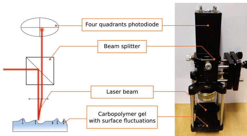
Figure 2. Free surface fluctuation technique illustration
