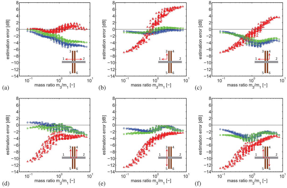
Figure 2. Estimation error as a function of the mass ratio m_3/m_1 for the average vibration reduction indices over 200 – 1250 Hz of the double wall H-junction, when modeled as an equivalent X-junction with single walls having the same thickness/density (blue), double thickness (red) or double density (green) compared to a single cavity wall leaf of the H-junction.
