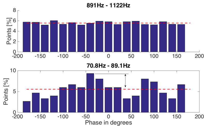
Figure 2. Histograms from analysis of room's transfer function phase at low (bottom), and high (top) frequencies. The red lines indicate the population counting in the case of a perfect uniform distribution. The proposed measure is indicated in the graphic displayed at the bottom.
