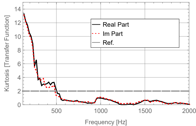
Figure 3. Average Kurtosis of real and imaginary parts from 15 transfer functions measured in the larger ( 108.5m^3 ) room.
