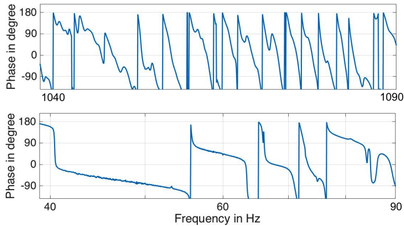
Figure 1. Room's transfer function within a 50 Hz window, at low (bottom), and high (top) frequencies. From measurements in a 108.5m^3 reverberant room.
