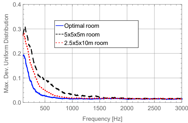
Figure 6. Maximum deviation from uniform distribution averaged from 15 transfer functions for three idealized rooms with same volume ( 125 \text{ m}^3 ), and reverberation time (10 seconds).
