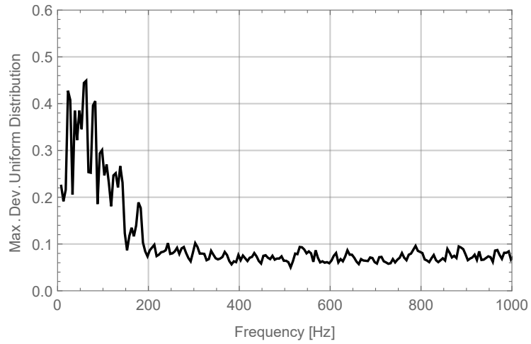
Figure 4. Maximum deviation from uniform distribution averaged from 15 transfer functions measured in the larger ( 108.5m^3 ) room.
