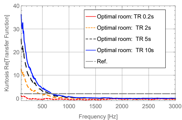
Figure 7. Kurtosis averaged from 15 transfer functions for the optimal room, with different reverberation times.
