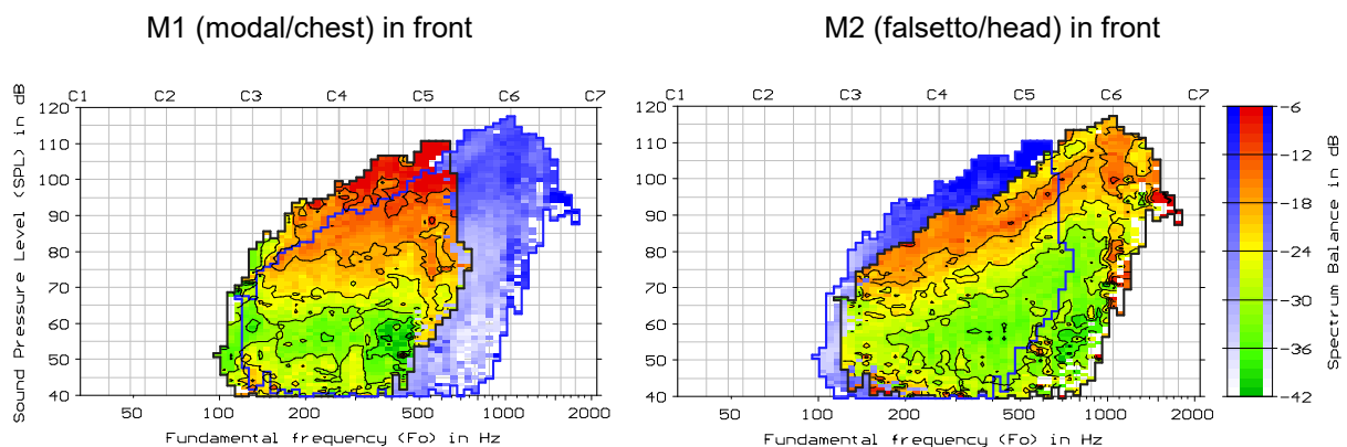
Figure 3. Maps of the spectrum balance SB, derived by averaging the power spectra over the union set of the VRP areas, for 12 trained female voices.
