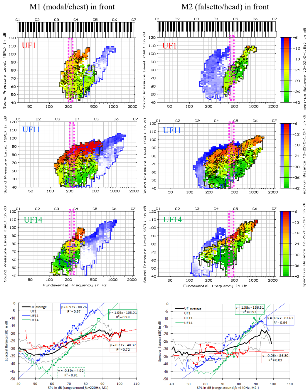
Figure 2. Inter-subject variability: top three rows: voice maps of SB, three untrained female subjects in M1 (modal/chest voice, left) and M2 (head/falsetto voice, right). The spectrum balance SB is mapped to colour (vertical bars). Bottom row: SB as function of SPL in M1 at 220 Hz (left) and in M2 at 440 Hz (right), at the sections indicated by dotted rectangles in the voice maps. Regression lines are based on the parts of the curves with marker dots.
