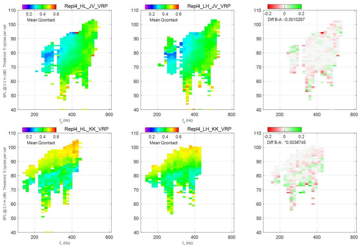
Figure 1: Reproducibility: aggregated voice field maps of the EGG contact quotient of two trained female singers singing the same short song many times at various dynamic levels p-mf-f . Top, a classical soprano; bottom, a jazz singer, singing in a lower key. The left and center panels show outcomes from disjunct replicated sets of the same task. The right panels show the small differences between the two sets. Each cell (1 semitone \times 1 dB) contains a contact quotient average over typically hundreds of phonatory cycles.
