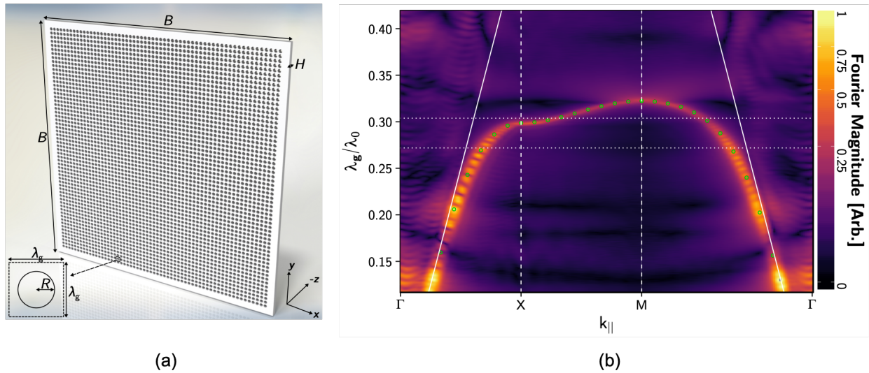
Figure 1. Schematic and mode dispersion of square hole array: (a) acrylic plate schematic, the sample has side lengths B = 560.00 mm, hole depth H = 9.60 \pm 0.23 mm, hole radius R = 3.25 \pm 0.05 mm, with an x/y grating pitch \lambda_g = 8 mm. (b) measured dispersion of the hole array sample between points of high lattice symmetry, obtained from the spatial Fourier transforms of the pressure fields of the acoustic mode propagating on the surface.
