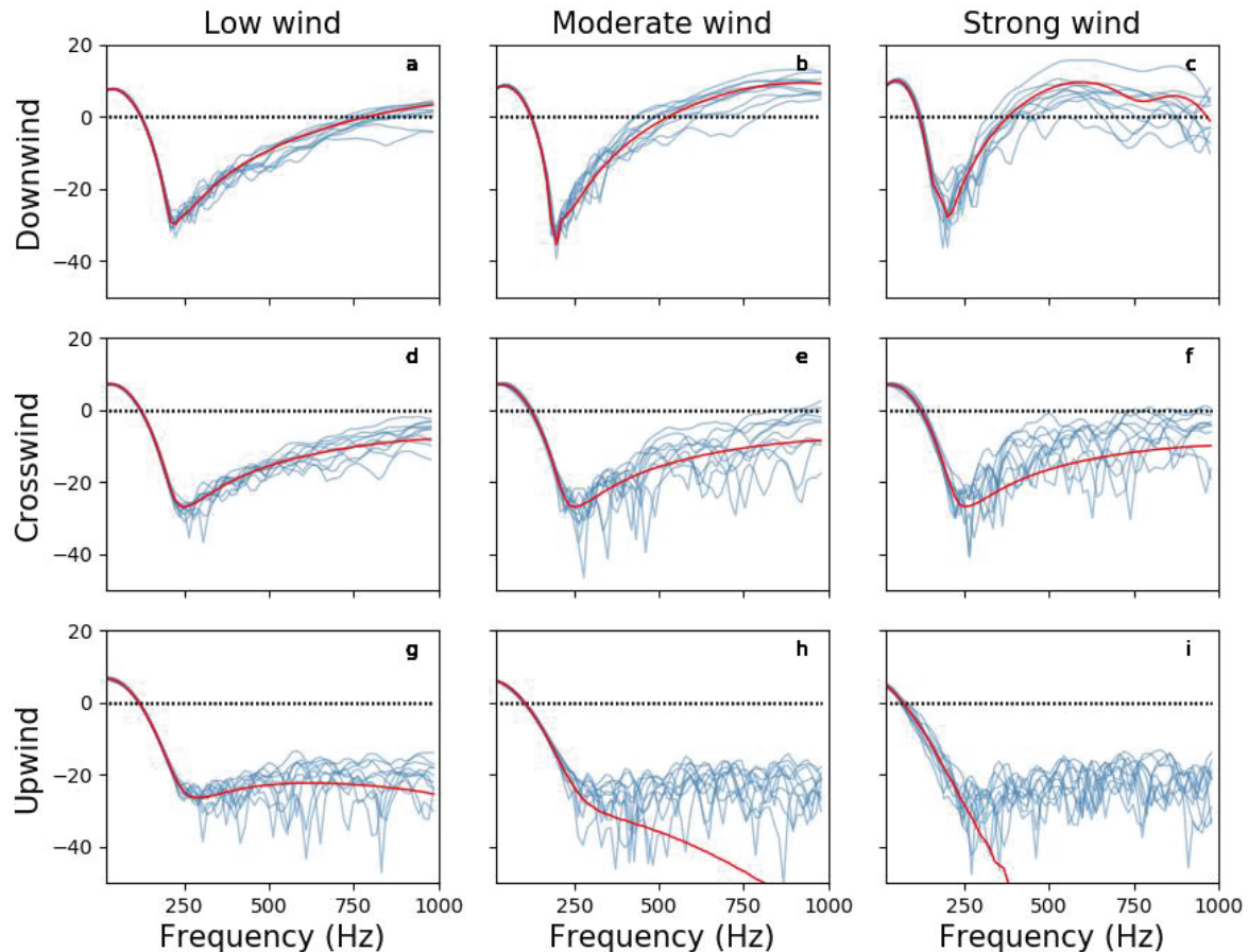
Figure 2 – Environmental gain (in dB, taken as 20 \log_{10}(A_{\text{FDTD}}/A_{\text{FF}}) , with A_{\text{FDTD}} the amplitude of the transfer function simulated with the environment, and A_{\text{FF}} the amplitude of the free field transfer function), with varying wind directions and strengths, at range 200 m and height 2 m. The dotted line is in free-field, the red line is without turbulence, the blue lines show 10 simulations with turbulence.
