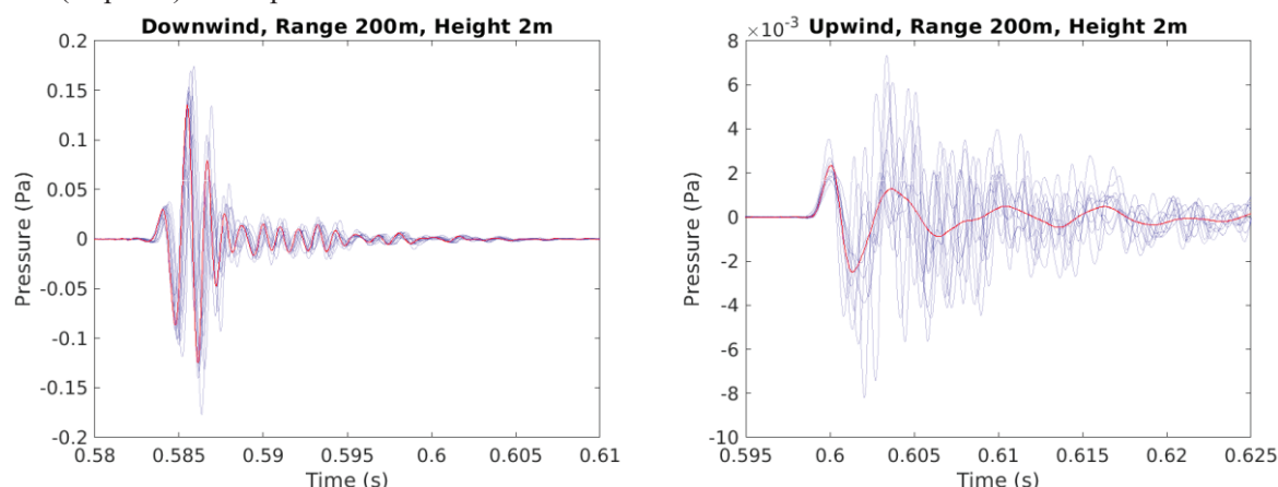
Figure 3 – Acoustic signatures derived from the database for an impulse sound at range 200 m. The red line is without turbulence, the blue lines show 10 simulations with turbulence.
