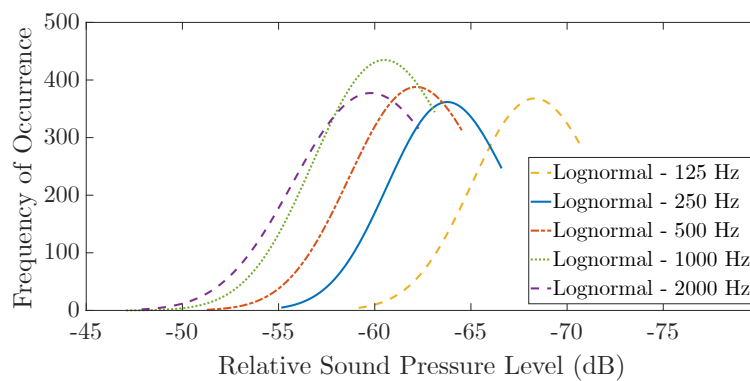
Figure 7. Frequency of occurrence of relative sound pressure level in distance of 500m in turbulent atmosphere with a sample rate of n = 5000 and distribution fit of data truncated at the mean value for analyzed frequencies.
