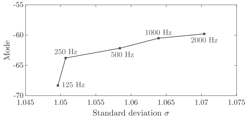
Figure 8. Ratio of mode and standard deviation of the lognormal distributions for analyzed frequencies.
