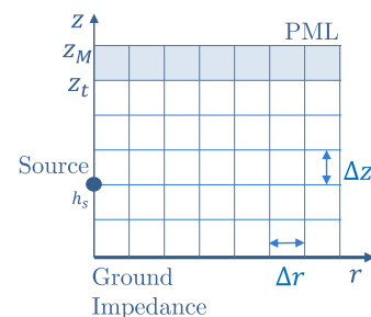
Figure 2. Sound field with discretization and boundary conditions.
