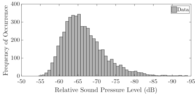
Figure 5. Frequency of occurrence of relative sound pressure level in distance of 500m in turbulent atmosphere with a sample rate of n = 5000 .
