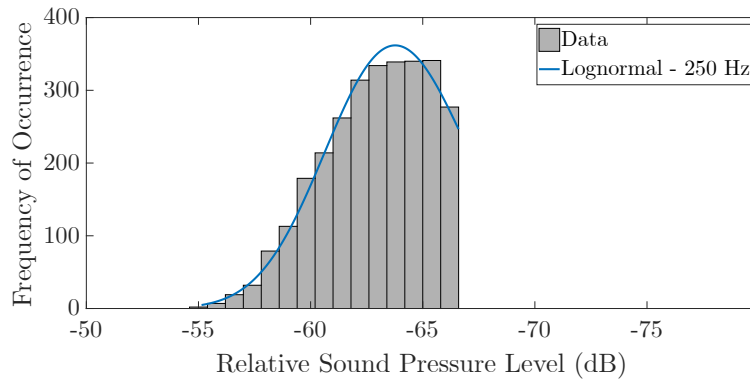
Figure 6. Frequency of occurrence of relative sound pressure level in distance of 500m in turbulent atmosphere with a sample rate of n = 5000 and distribution fit of data truncated at the mean value.
