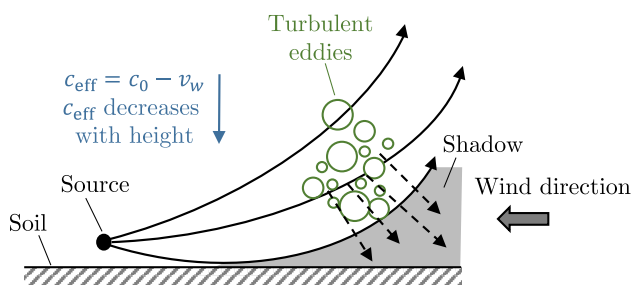
Figure 1. Refraction of sound waves and scattering at turbulent eddies into the shadow zone.
