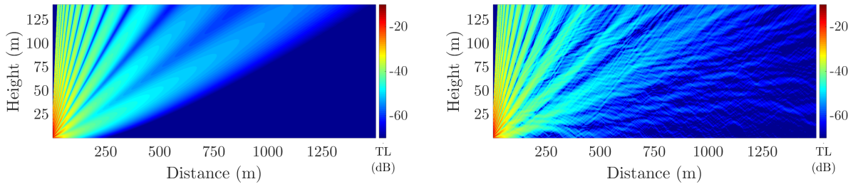
Figure 4. Transmission loss in non-turbulent (left) and turbulent (right) upward refracting atmosphere at 250Hz.
