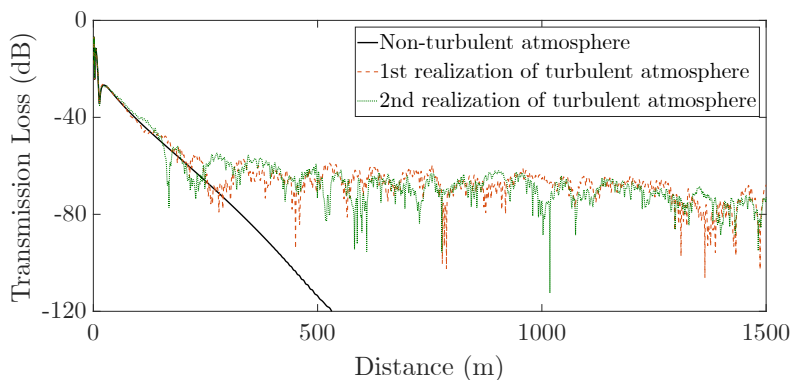
Figure 3. Transmission loss in direction of propagation in an upward refracted atmosphere.
