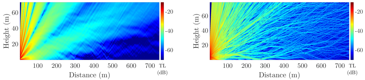
Figure 9. Transmission loss in turbulent upward refracting atmosphere at 125 Hz (left) and at 2000 Hz (right).
