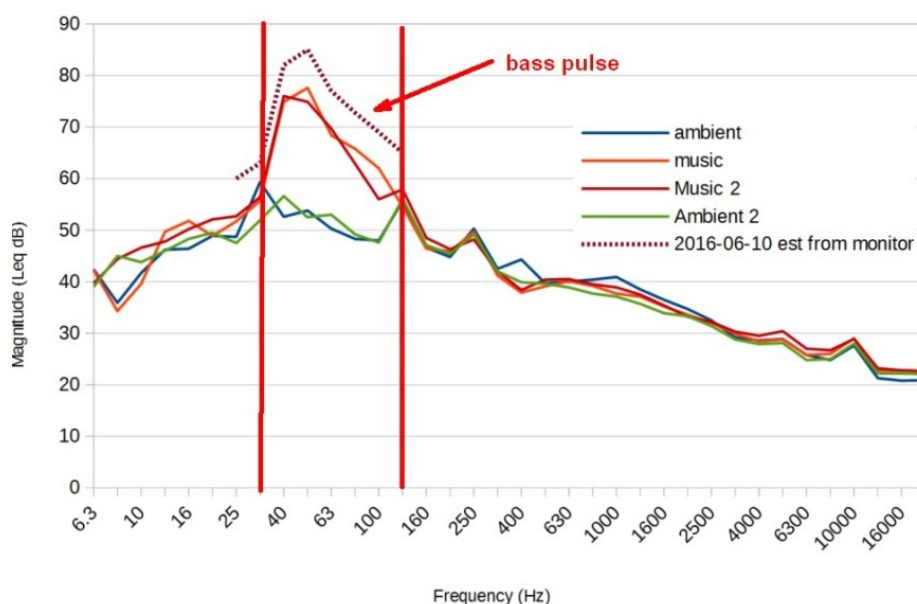
Figure 2: Outdoor measurements 29m (95ft) from a club in an apartment complex 12:00am versus ambient conditions.
