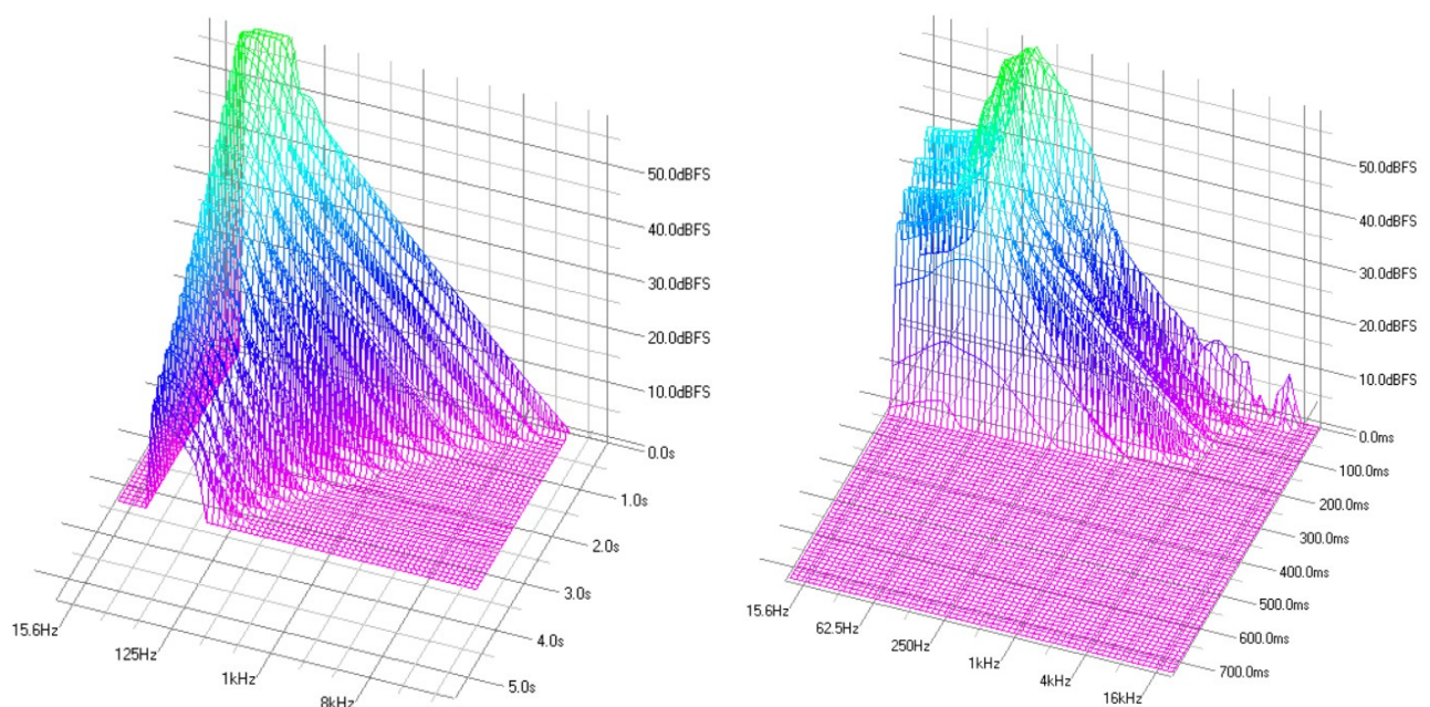
Figure 3: Waterfall analysis of two bass drops. Left, a well ordered oscillating 3 second drop; Right, a 0.2 second drop with some electronic effects. In both cases, the signal shifts to lower frequency over time.
