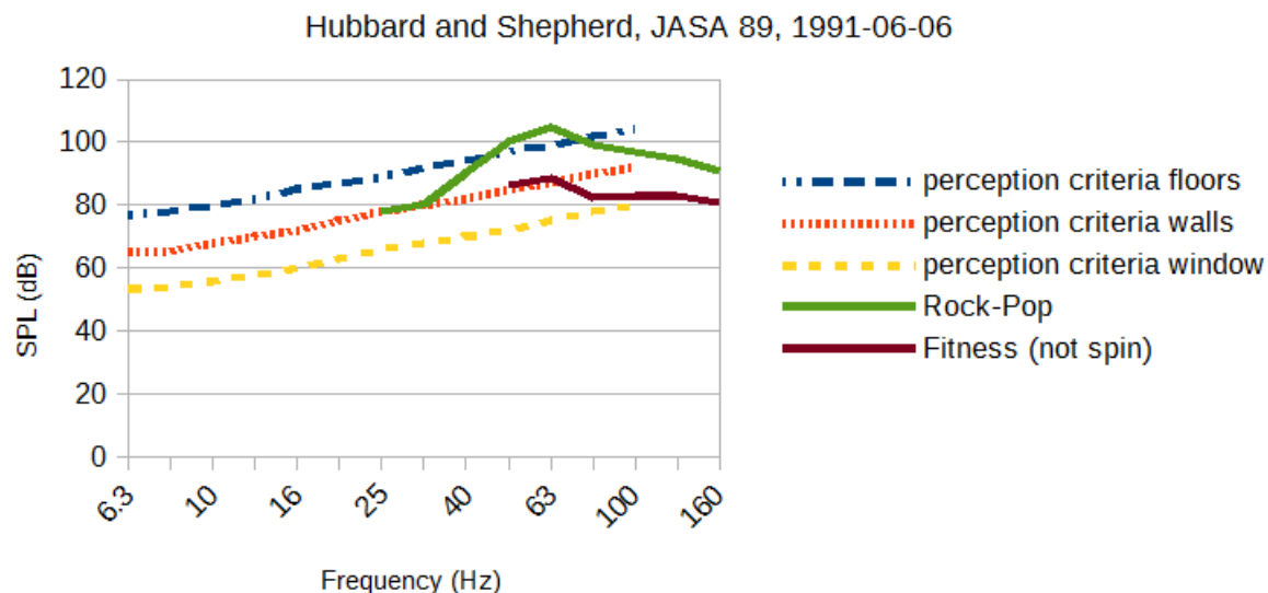
Figure 4: NASA thresholds of airborne sound levels producing perceived induced structural vibrations. Rock-pop curve extracted from Larsen(6) and author’s field data, fitness is typical ambient conditions for a fitness facility. Note that “spin” (in-place bicycle class) can exceed the fitness level significantly (up to 10dB). Both typical field conditions can induce structureborne sound.
