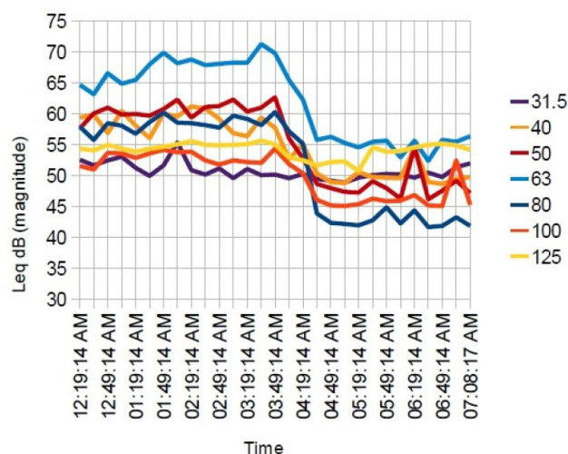
Figure 1: Third octave band measurements of Leq in a bedroom on 5 th floor of condominium above an open stairwell with club on 1 st floor, Note the drop in level of 15dB when the club closes at 4:00am.
