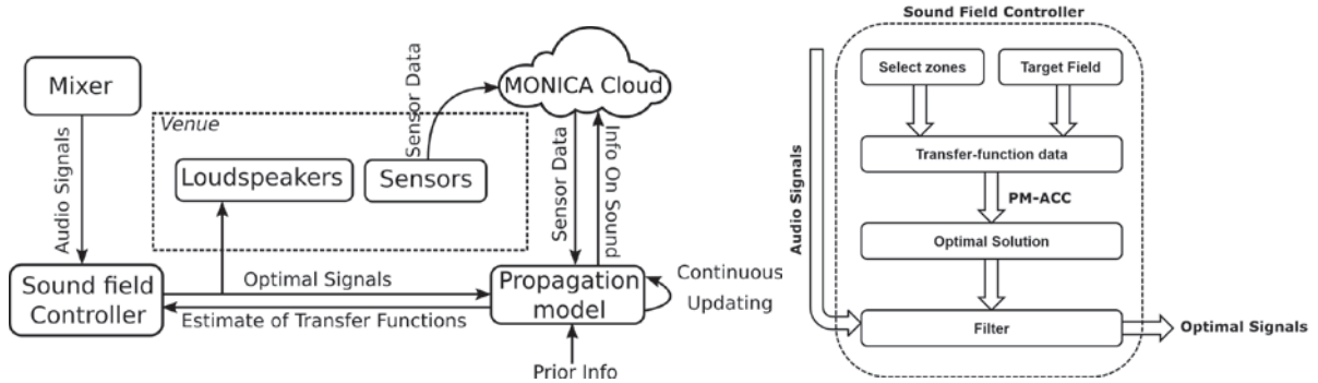
Figure 1 – Left: Information flow in the sound field control system, from [1]. Right: Signal processing flow of the Sound Field Controller module.
