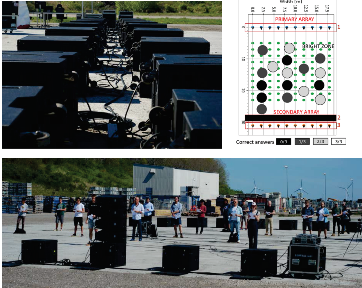
Figure 4 – The full-scale pre-test at Refshaleøen. Upper-left: Double array of secondary subwoofers. Upper-right: Result of the preliminary listening test in the bright zone (audience area). Darker circle means the subject failed to discriminate the difference. Lower: In the front the primary subwoofer array and complementary mid-high frequency line array, in the back the secondary subwoofer array. A listening test is conducted in the audience area (bright zone).
