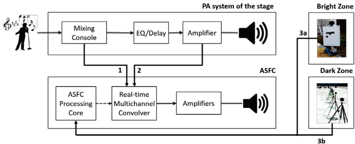
Figure 3 – Monitoring/Playback signal chain configuration of the ASFC system.
