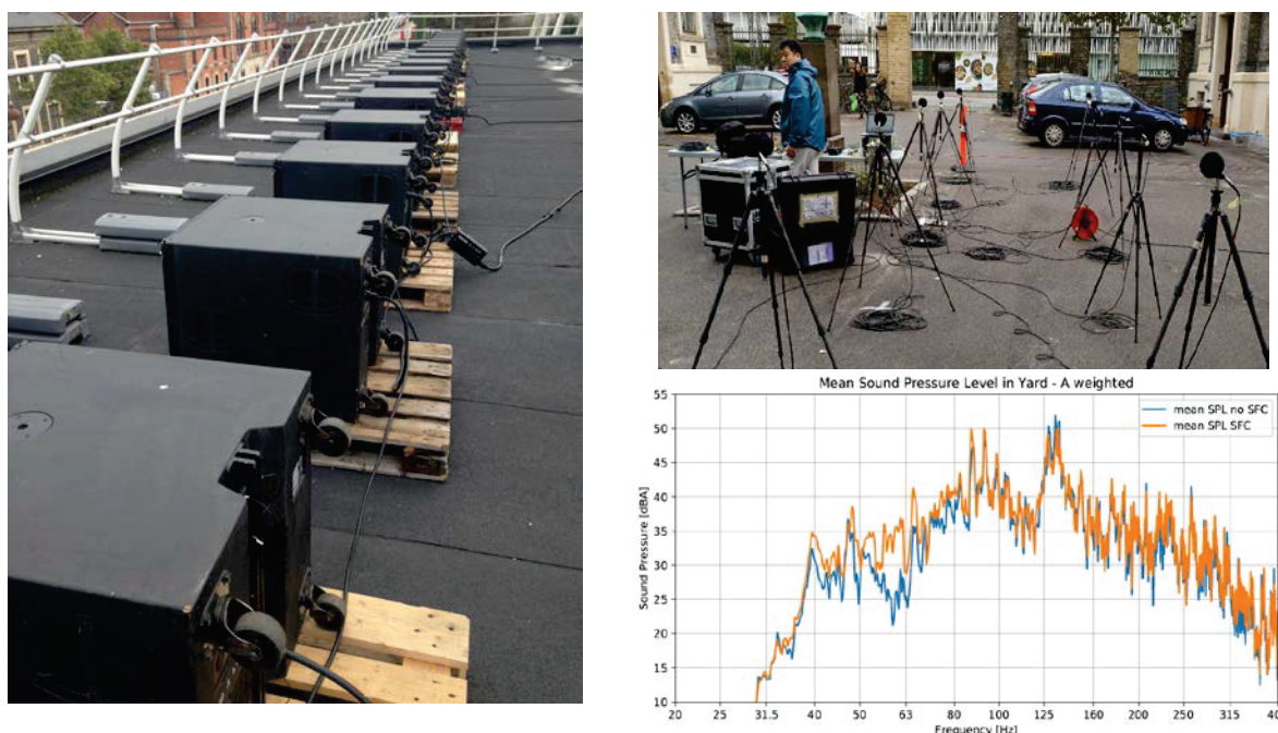
Figure 7 – The full-scale pilot test at Tivoli. Left: The subwoofer secondary array on the roof. Right-top: Microphone positions in the dark zone. Right-bottom: Average SPL in the dark zone.
