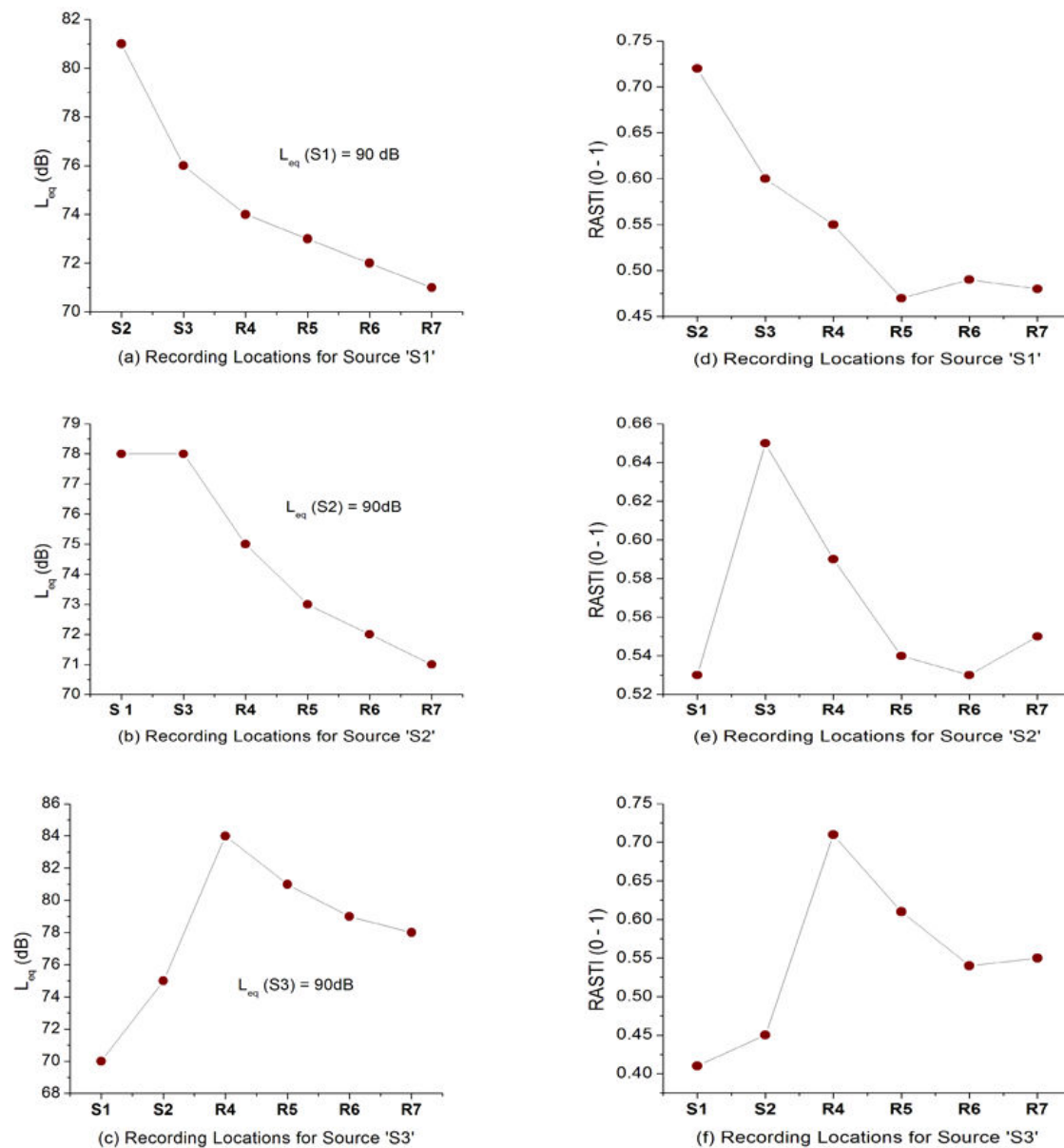
Figure 9 – Positional variance for L_{eq} and RASTI in St. Roque church.
