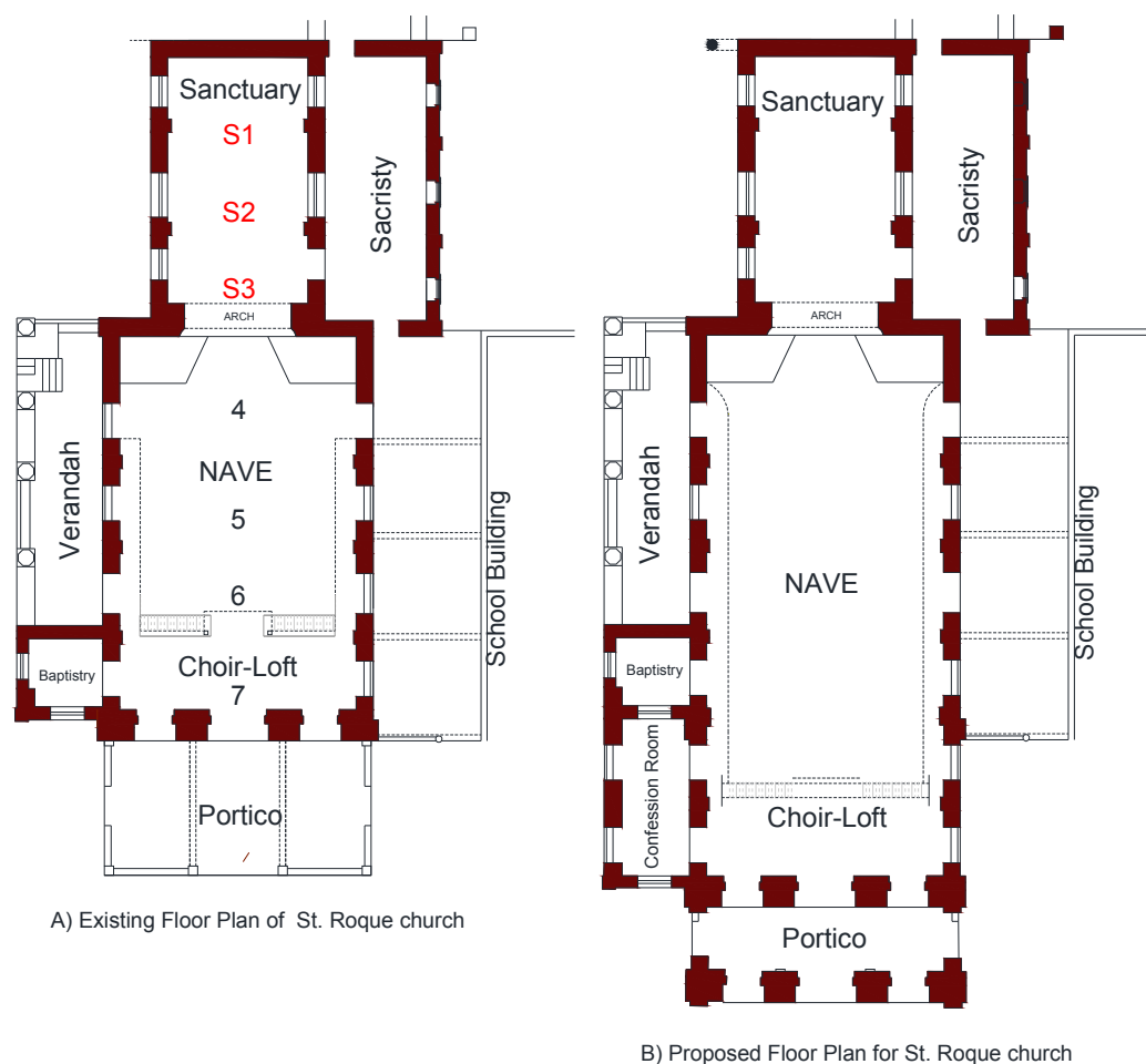
Figure 2 – a) Existing Floor Plan of St. Roque church with marked locations of sound sources (S1, S2, S3) and recording locations (S1, S2, S3, 4, 5, 6, 7) b) Floor plan of the Proposed expanded St. Roque church.
