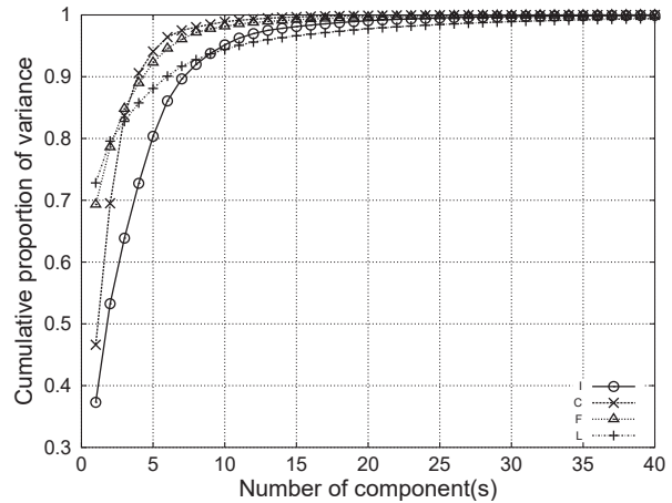
Fig. 1. Change in cumulative proportion of variance (CPV) with number of component in PCA.
