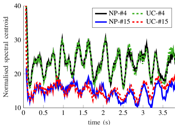
Figure 7. Comparison of the normalised spectral centroids between two different playing conditions for key 4 (C1) and 15 (B1).
