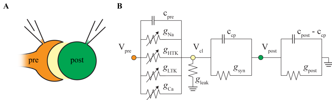
Figure 1 – Model circuit to simulate the prespike. (A) Drawing of the calyx of Held synapse. The calyx of Held terminal ('pre') covers a large area of the soma of its target neuron ('post'). In between is a small space, called the synaptic cleft, where membrane currents will flow during a presynaptic AP. (B) An electrical circuit for the capacitive and resistive currents that flow from the presynaptic membrane into the postsynaptic cell to generate a prespike.
