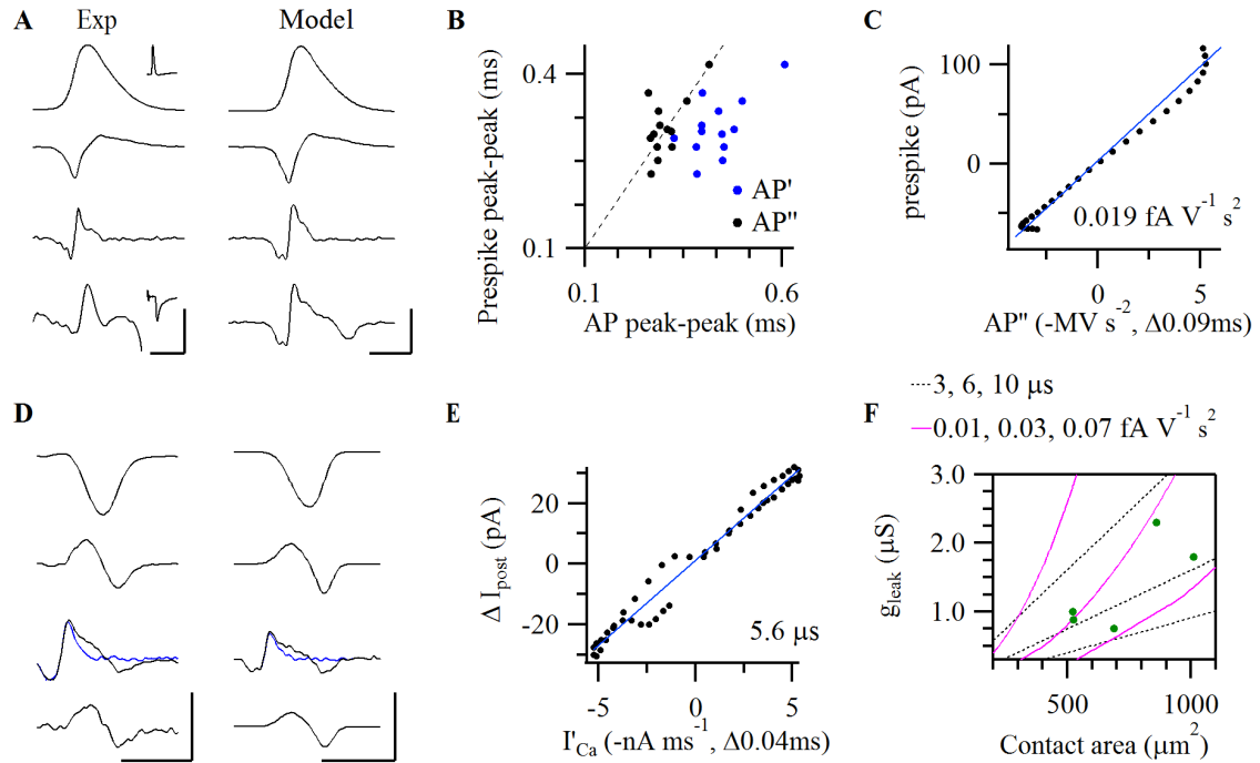
Figure 2 – Relation between the calyceal AP and the prespike. (A) Left column, from top to bottom : AP recorded from the calyx of Held, inverted first and second derivatives, and postsynaptic voltage clamp recording showing the accompanying prespike. Insets show on a longer time scale the same presynaptic AP (top) and the postsynaptic EPSC (bottom) elicited by the calyceal stimulation. Right : Only VGCCs-model results. Vertical scale bars (from top to bottom panels): 80 mV, 0.8 kV/s, 8 MV/s 2 , 0.2 nA. Horizontal: 0.5 ms. (B) Relation between the delay between the first negative and positive peak of the prespike and the first two peaks in the first (blue) and second (black) derivative of the presynaptic AP. Dashed line is the identity line. (C) Relation between the prespike and the second derivative shown in A. Maximum correlation was obtained when delaying the second derivative by 90 \mu s. Blue line shows the regression line with a slope ('transfer constant') of 0.019 \text{ fA V}^{-1} \text{ s}^2 . (D) Left column, from top to bottom : Presynaptic calcium current (after P/5 subtraction), its first derivative, postsynaptic currents (black) plus passive prespike (blue), difference between active and passive prespike. Right : corresponding model results. Vertical scale bars: 2 nA, 15 nA/ms, 0.15 nA, 0.1 nA. Horizontal: 1 ms. (E) Relation between the calcium component of the prespike and the first derivative of the presynaptic calcium current shown in D. Maximum correlation was obtained when delaying the first derivative by 40 \mu s. Blue line shows regression line with a slope ('time constant') of 5.6 \mu s. (F) Relation between the contact area and the cleft leak conductance for different values of the transfer constant (magenta lines) and the time constant (black lines). Green dots show the values of the model for the five double VC recordings calculated from the measured transfer and time constants. Calcium current density was 0.11 \text{ nS } \mu\text{m}^{-2} in the simulations.
