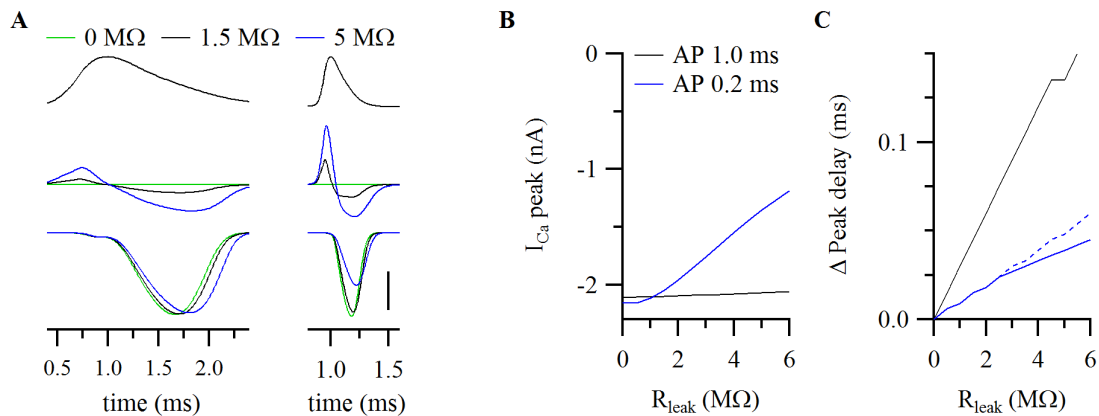
Figure 3 – Impact of the cleft potential on presynaptic calcium currents. (A) Simulation of the impact of a slow and a fast AP (top; FWHM: left 1.0, right 0.2 ms) on the cleft potential (middle) and the presynaptic calcium current (bottom) at three leak resistances, as indicated above the figure. Scale bar: 90 mV, 14 mV, 1 nA. (B) Relation between peak calcium currents and leak resistance for the two APs. Driving force increases slightly (not shown). (C) The change in delay between the calcium peak current and the AP for the two APs (solid line). The dashed line shows the delay after correcting for the decrease in the calcium current shown in B. Calcium conductance density was 0.1 and 0.2 \text{nS } \mu\text{m}^{-2} for the slow and fast AP, respectively.
