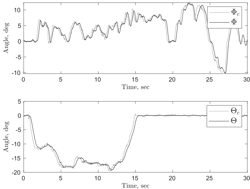
Figure 9. Attitude controller performance in hover flight (experiment).
