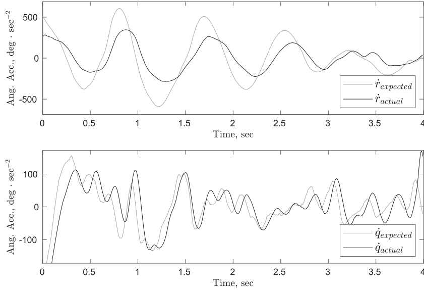
Figure 8. Comparison of expected and actual angular accelerations in hover flight (experiment).
