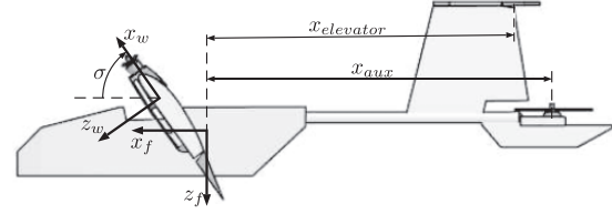
Figure 2. Side view of the aircraft.
