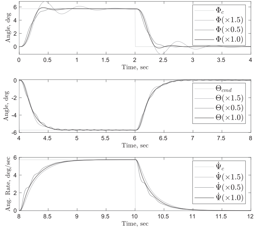
Figure 6. Attitude controller performance in hover flight (simulation).
