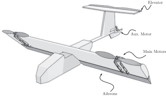
Figure 1. Example tiltwing aircraft in hover configuration.
