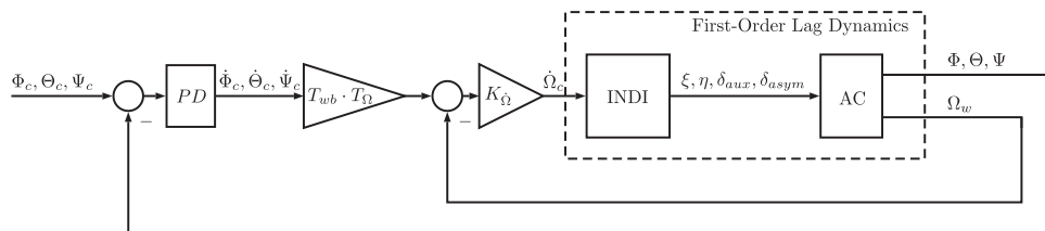
Figure 4. Attitude controller loop.
