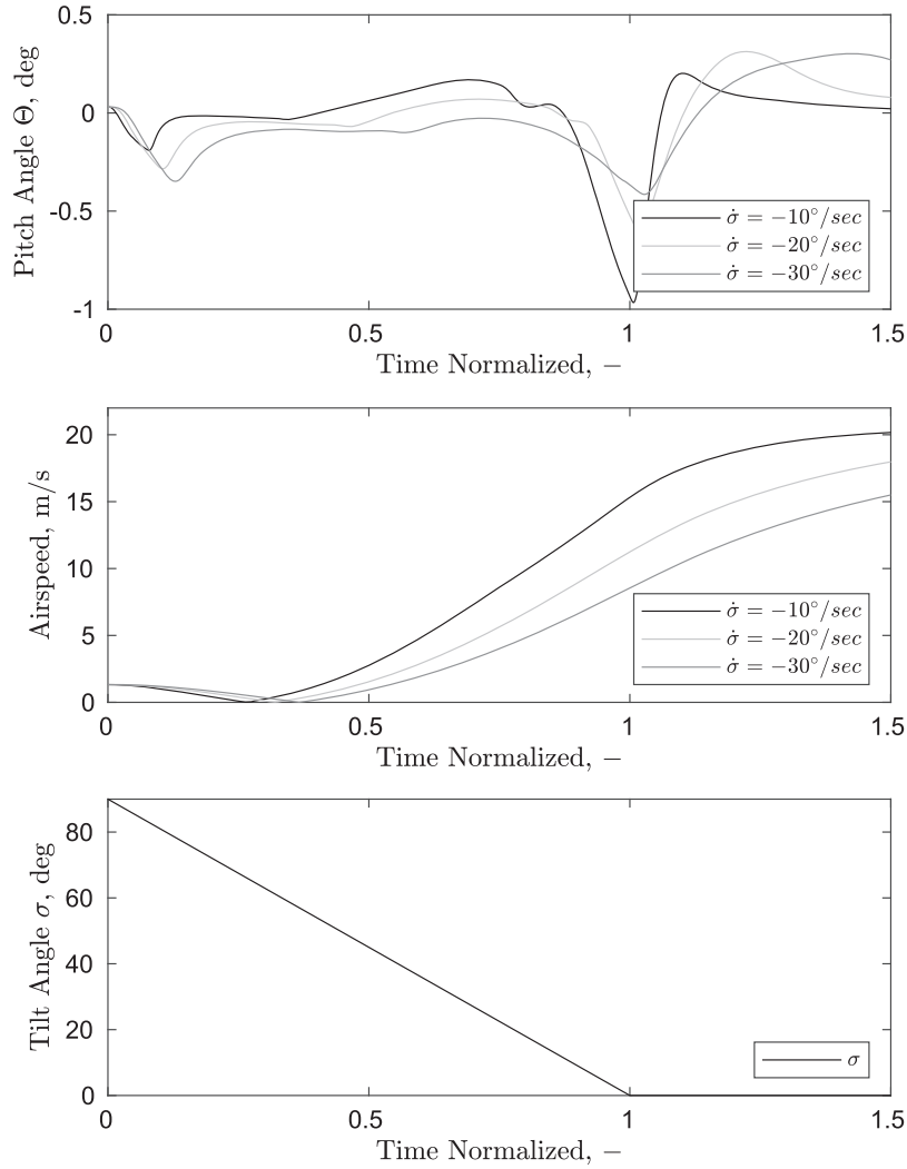
Figure 5. Pitch angle error during transition at different transition speeds (simulation).
