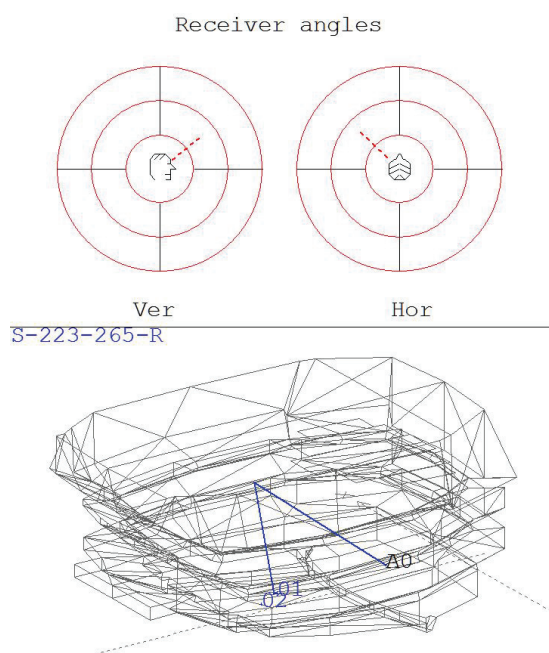
Figure 12: Origin of the reflection showed in Figure 11 as predicted during the design stage for the SR pair A0-02. It has a delay of 61 ms after the direct sound
