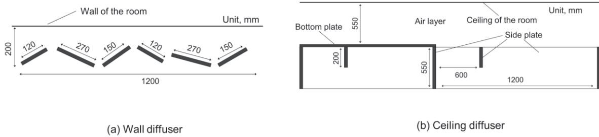
Figure 2 – Cross sections for (a) Wall diffuser and (b) Ceiling diffuser.
