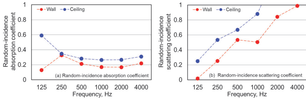
Figure 4 – Acoustic characteristics of the diffusers. (a) Random-incidence absorption coefficient and (b) Random-incidence scattering coefficient.
