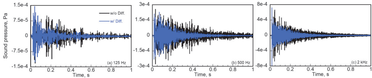
Figure 6 – Comparisons of 1/1 octave limited impulse responses at R5 up to 1.0 s compared between the scaled rehearsal room without and with diffusers at (a) 125 Hz, (b) 500 Hz and (c) 2 kHz.
