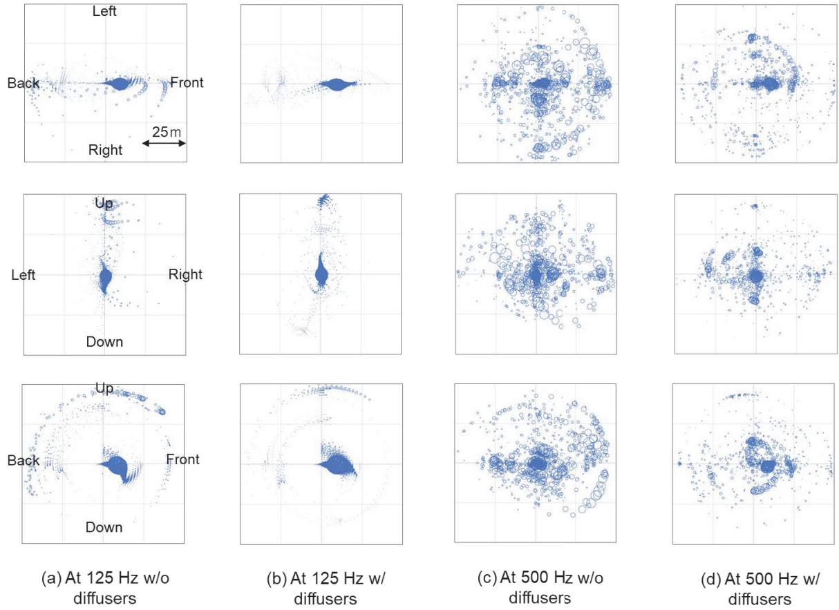
Figure 9 – Visualizations of virtual image source distributions for four conditions:(a) At 125 Hz without diffusers, (b) At 125 Hz with diffusers, (c) At 500 Hz without diffusers and (d) At 500 Hz with diffusers.
