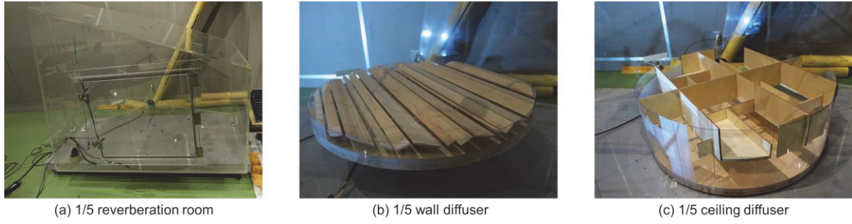
Figure 3 – 1/5 scaled models for the absorption and scattering measurements: (a) 1/5 reverberation room, (b) 1/5 wall diffuser and (c) 1/5 ceiling diffuser.
