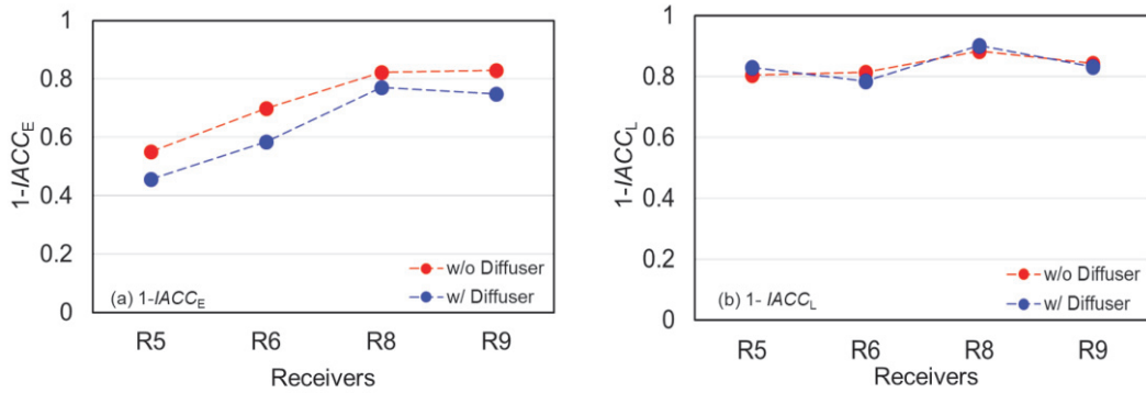
Figure 8 – Comparisons of IACC s between the rehearsal room without and with diffusers. (a) 1-IACC_E and (b) 1-IACC_L .
