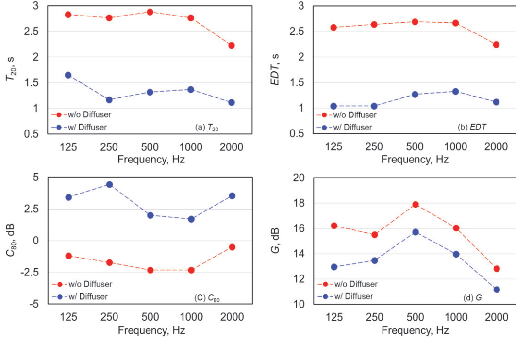
Figure 7 – Comparisons of acoustic parameters averaged at 9 receivers between the rehearsal room without and with diffusers. (a) T_{20} , (b) EDT, (c) C_{80} and (d) G .
