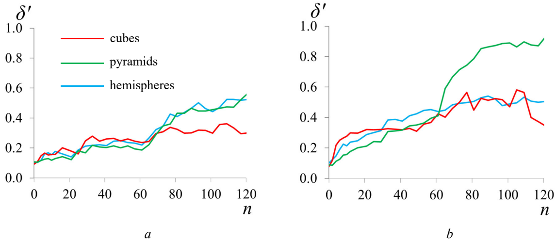
Figure 5 – Measured coefficient \delta' at 4kHz (a) and 8 kHz (b) in dependence on the number of the diffusers n
