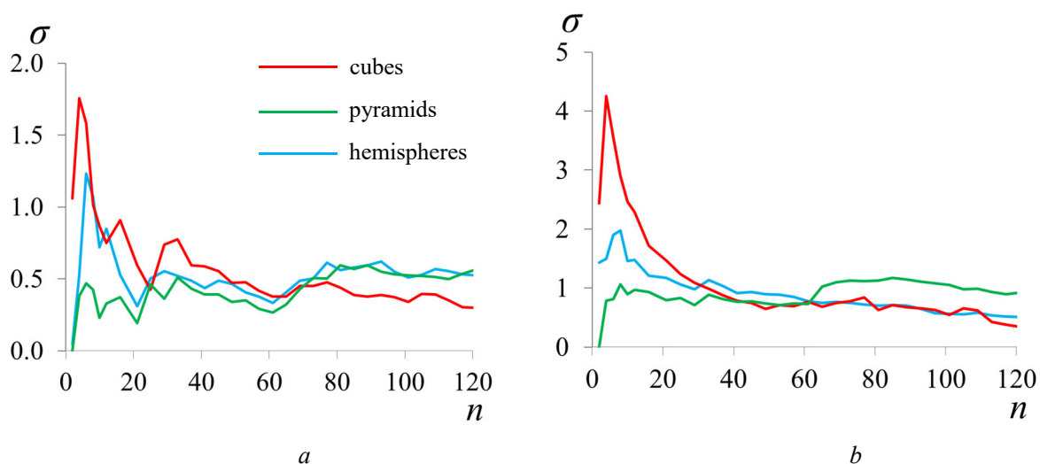
Figure 6 – Scattering cross section of one diffuser at 4kHz (a) and 8 kHz (b) in dependence on the number of the diffusers n
