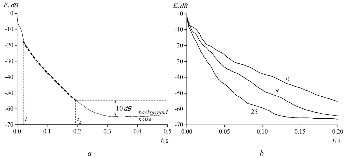
Figure 3. The measured decay curves in the model experiment (Fig. 2): a - an example of approximation of the measured decay curve by the theoretical dependence (9), indicated by a dotted line; b - decay curves measured in a room without scattering cubic elements (curve 0), as well as with 9 and 25 elements.
