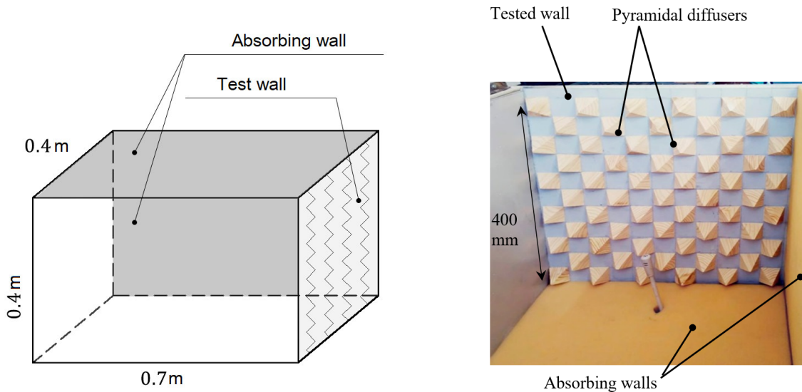
Figure 2 – A scale-model room
