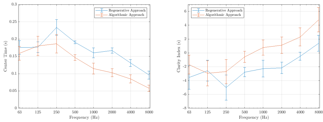
Figure 10 – Position-averaged Center Time (left) and Clarity Index (right) (CCS)
