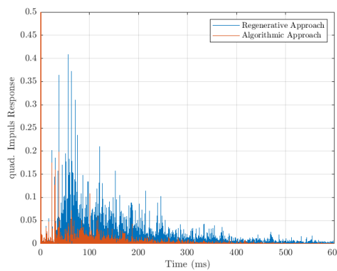
Figure 9 – Reflectograms of both approaches (direct energy scaled to 1, zoomed in to 0.5 and 600ms)
