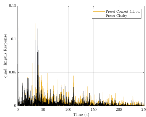
Figure 15 – Impulse response of tunings with different clarity (direct energy scaled to 1, zoomed in to 0.15 and 250ms) (ACH)
