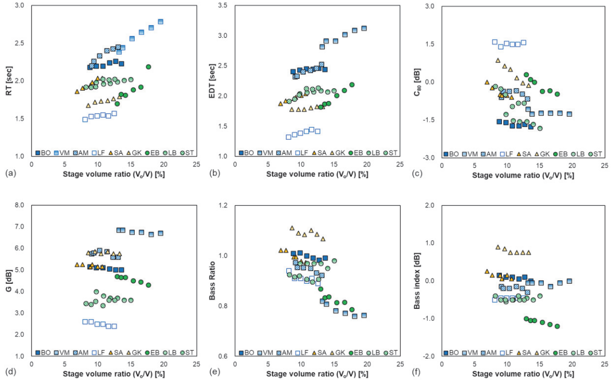
Figure 1 – Acoustic parameters according to the stage volume ratio ( V_o/V ) (a) RT, (b) EDT, (c) C80, (d) G, (e) Bass Ratio, (f) Bass index
