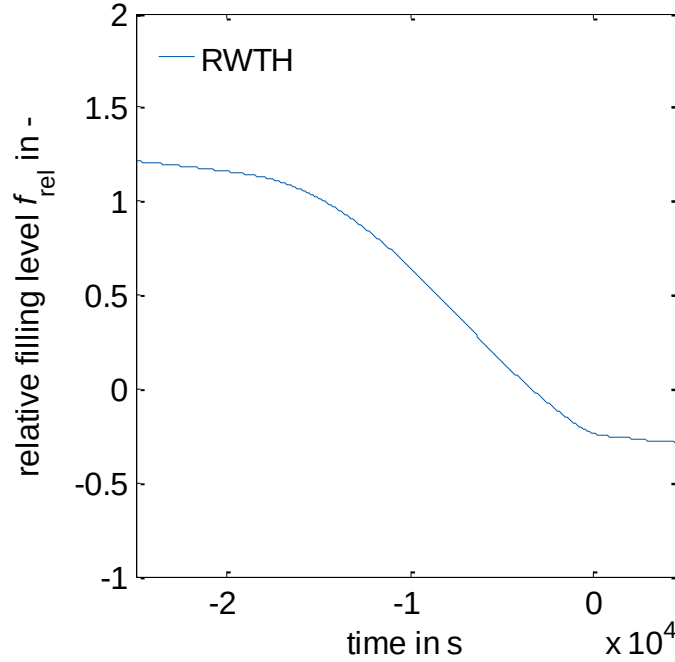
Fig. SI13: Relative filling level f_{\text{rel}} detected optically in the experimental setup at RWTH for the experiment with parameter set lowDF shown in Fig. 4.
