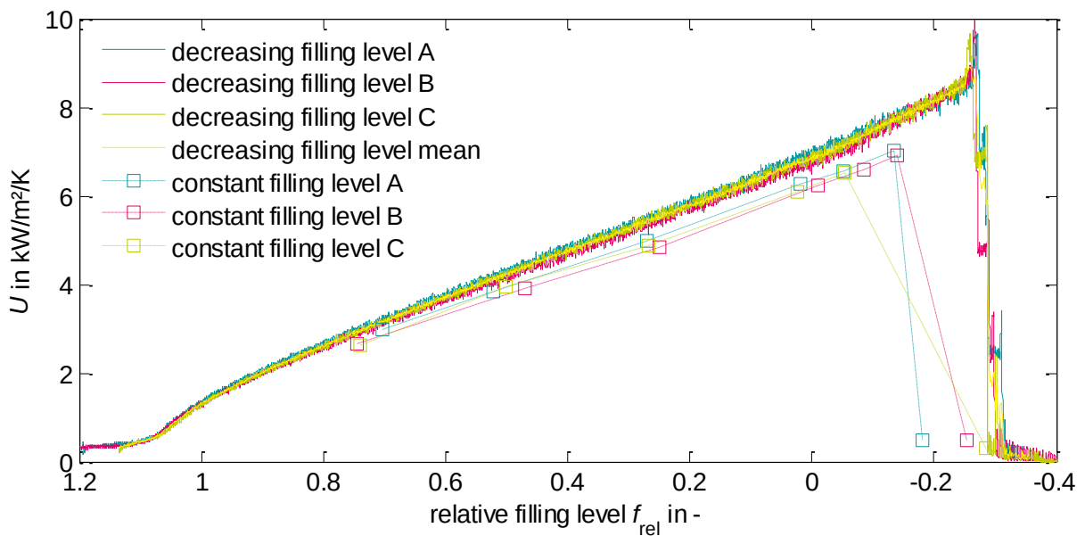
Fig. 6: U -values for experiments with continuously decreasing filling level (for each repetition A-C and arithmetic mean of A-C) and constant filling level (for each repetition A-C) plotted over relative filling level f_{\text{rel}} . Operating conditions of evaporator were according to Table 4. Condenser temperature was set to 10 °C. Data points of experiments with constant filling levels are connected by a dashed line to mark subsequently recorded data points.
