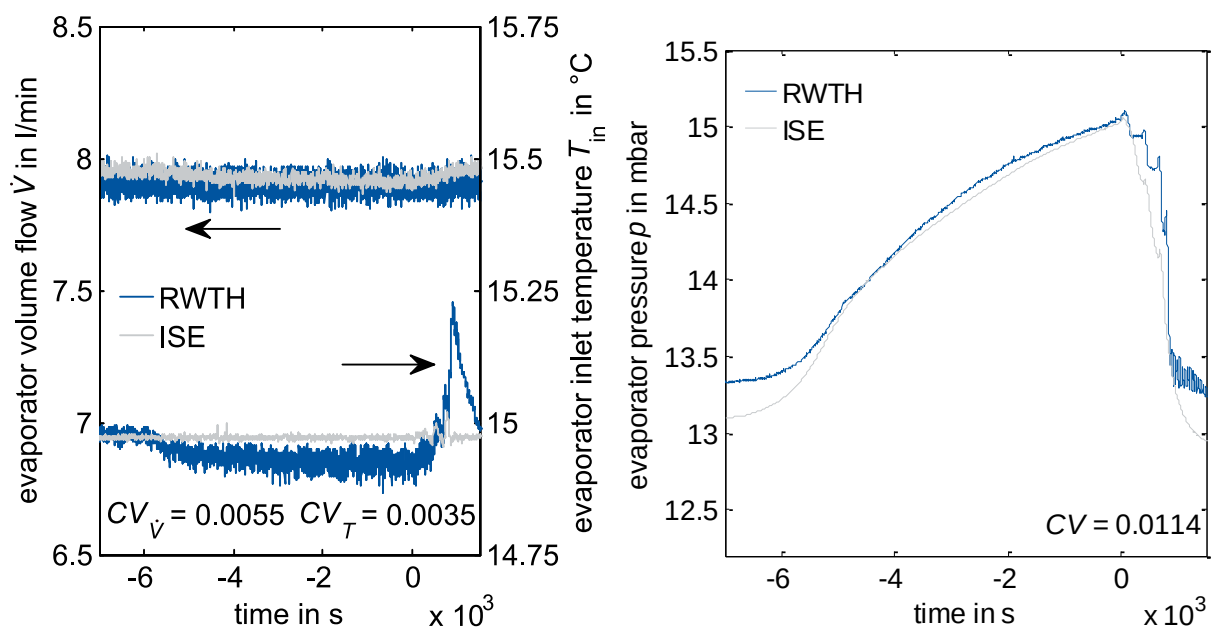
Fig. S18: Operating conditions for experiments with parameter set highDF plotted over time. Left: evaporator volume flow \dot{V} and inlet temperature T_{in} , right: evaporator pressure p . Both experiments
