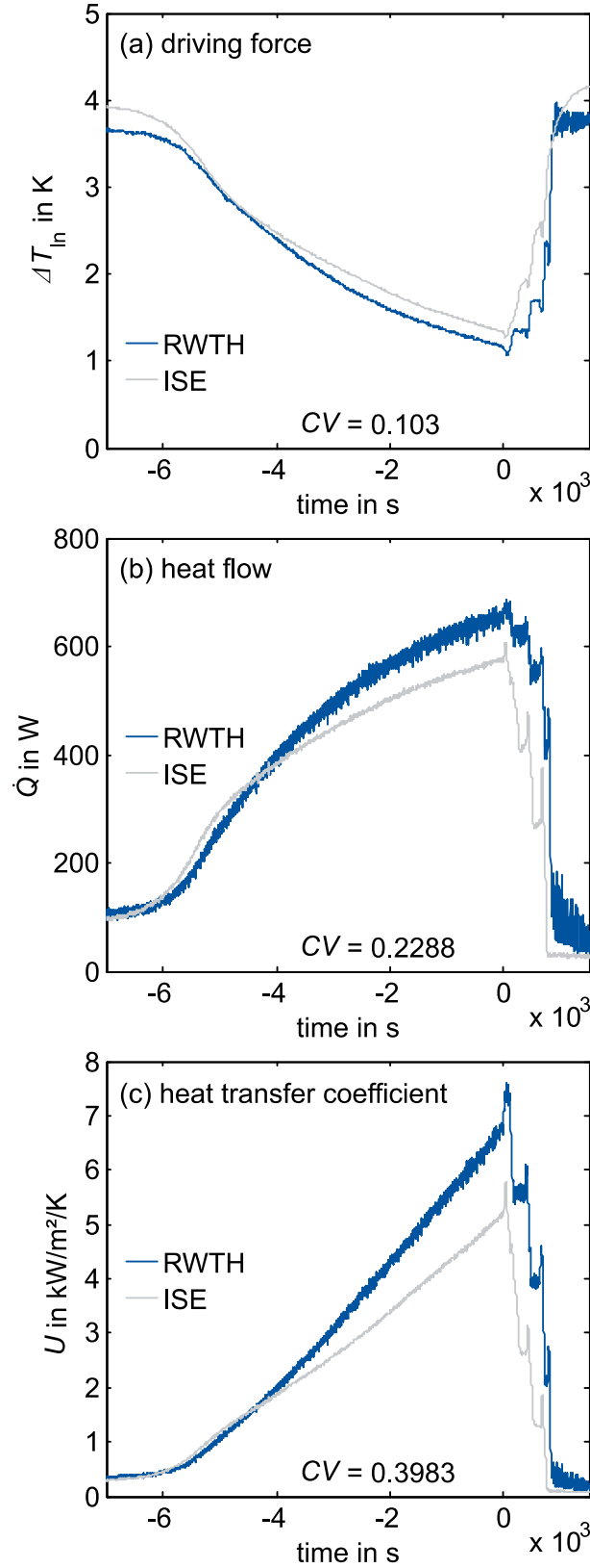
Fig. 5: Driving force \Delta T_{\text{in}} (a), heat flow \dot{Q} (b) and overall heat transfer coefficient U (c) plotted over time for experiments with parameter set highDF (Table 3). Both experiments (RWTH and ISE) are synchronized at the end of the experiment ( t=0 ) when the first tube loses contact to the refrigerant pool. The coefficient of variation CV (Eq. (7)) is given in each plot to quantify the deviation between the experiments at RWTH and ISE.
