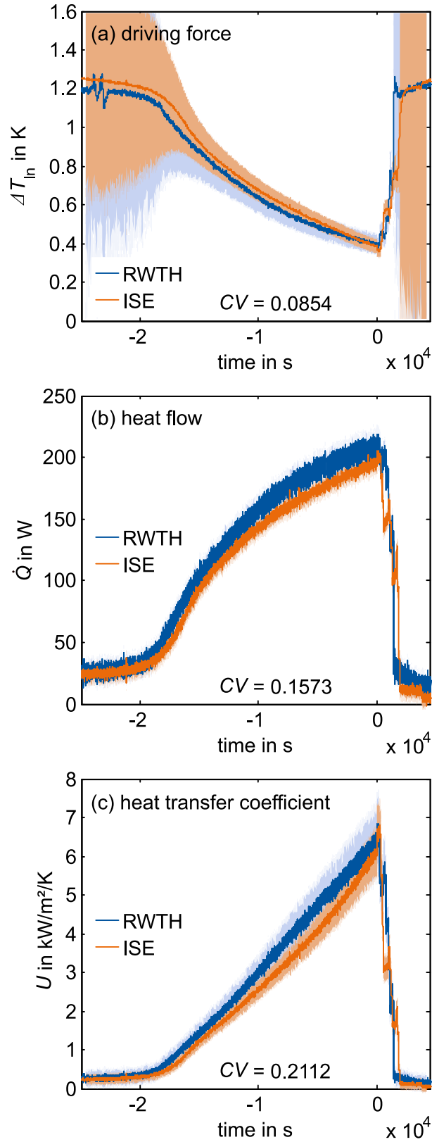
Fig. S110: driving force \Delta T_{in} (a), heat flow \dot{Q} (b) and heat transfer coefficient U (c) shown in Fig. 4 together with uncertainties of measurement (shown in Fig. S19) in background for experiments with parameter set lowDF plotted over time. Both experiments (RWTH and ISE) are synchronized at the end of the experiment ( t=0 ) when the first tube loses contact to the refrigerant pool.
