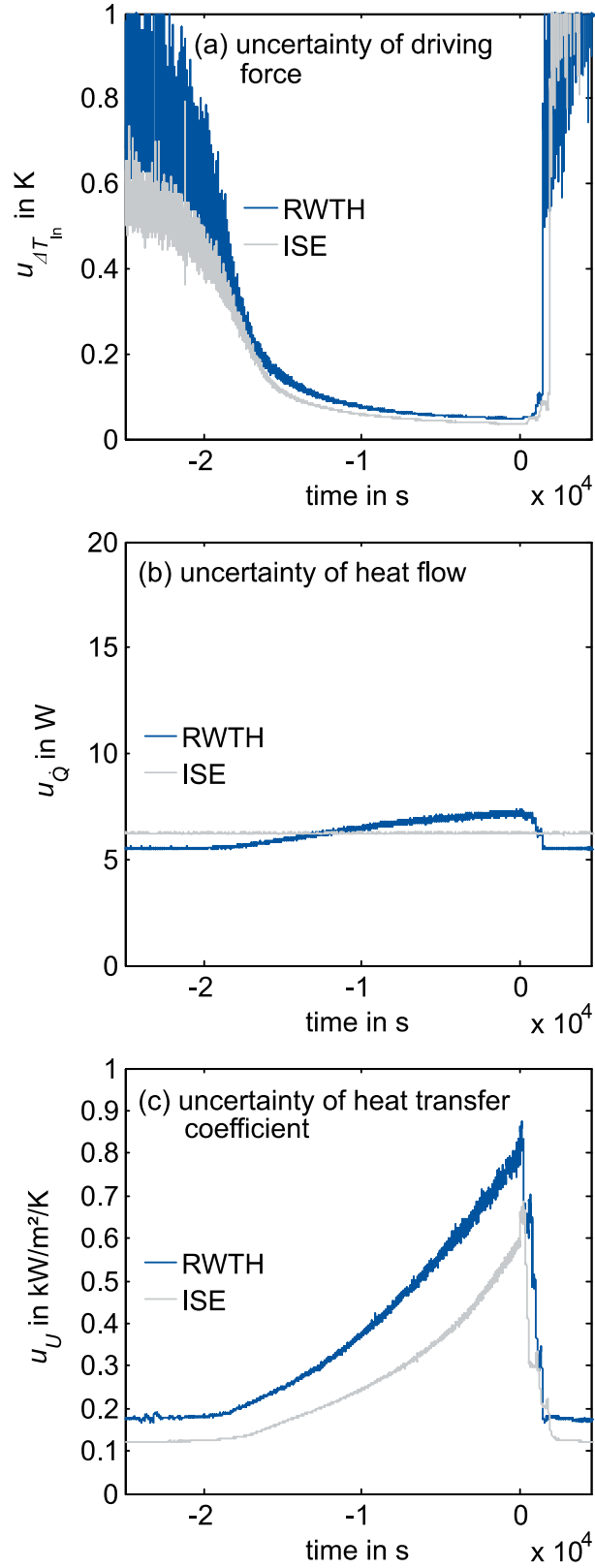
Fig. S19: Uncertainty in measurement for the quantities driving force \Delta T_{in} (a), heat flow \dot{Q} (b) and heat transfer coefficient U (c) shown in Fig. 4 for experiments with parameter set lowDF plotted over time. Both experiments (RWTH and ISE) are synchronized at the end of the experiment ( t=0 ) when the first tube loses contact to the refrigerant pool.
