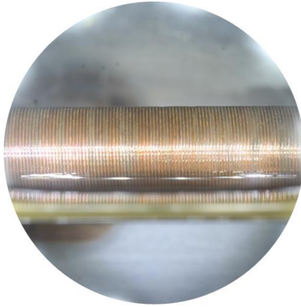
Fig. 1: Finned tube installed in the experimental setup at RWTH partly submerged in the refrigerant water during an experiment. The picture is taken through a round window on the side of the experimental setup. The other three tubes lie behind the shown tube. Capillary water between the fins of the tube as well as the menisci of water at the tube and at the window can be seen.
