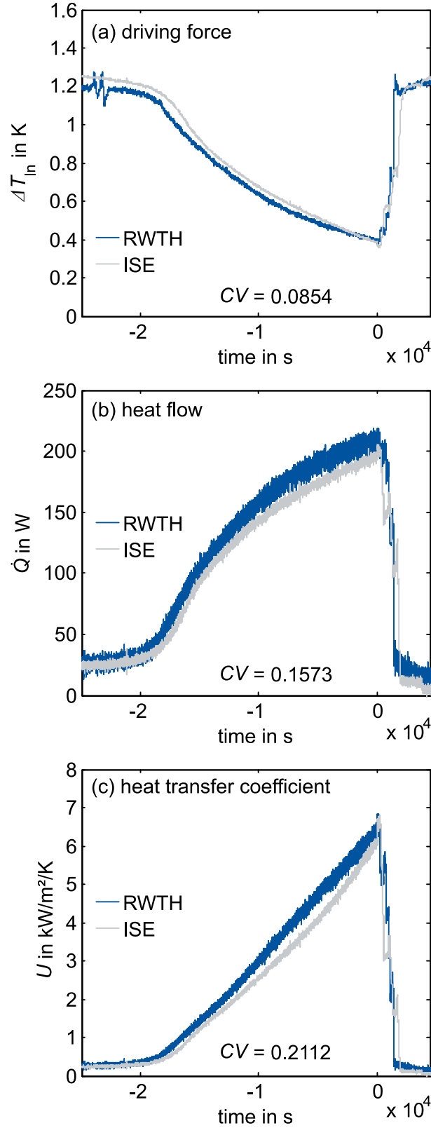
Fig. 4: Driving force \Delta T_{\text{in}} (a), heat flow \dot{Q} (b) and overall heat transfer coefficient U (c) plotted over time for experiments with parameter set lowDF (Table 3). Both experiments (RWTH and ISE) are synchronized at the end of the experiment ( t=0 ) when the first tube loses contact to the refrigerant pool. The coefficient of variation CV (Eq. (7)) is given in each plot to quantify the deviation between the experiments at RWTH and ISE.
