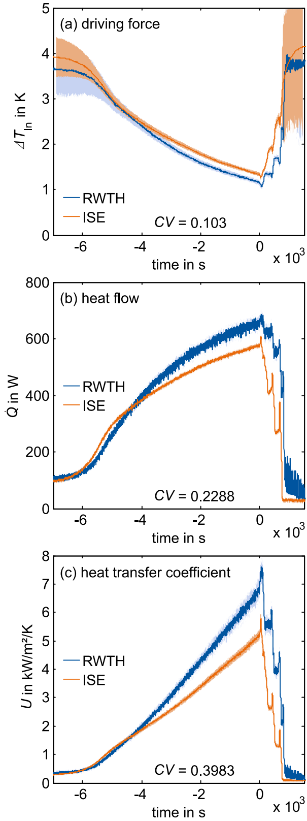
Fig. S112: Driving force \Delta T_{in} (a), heat flow \dot{Q} (b) and heat transfer coefficient U (c) shown in Fig. 5 together with uncertainties of measurement (shown in Fig. S111) in background for experiments with parameter set highDF plotted over time. Both experiments (RWTH and ISE) are synchronized at the end of the experiment ( t=0 ) when the first tube loses contact to the refrigerant pool.
