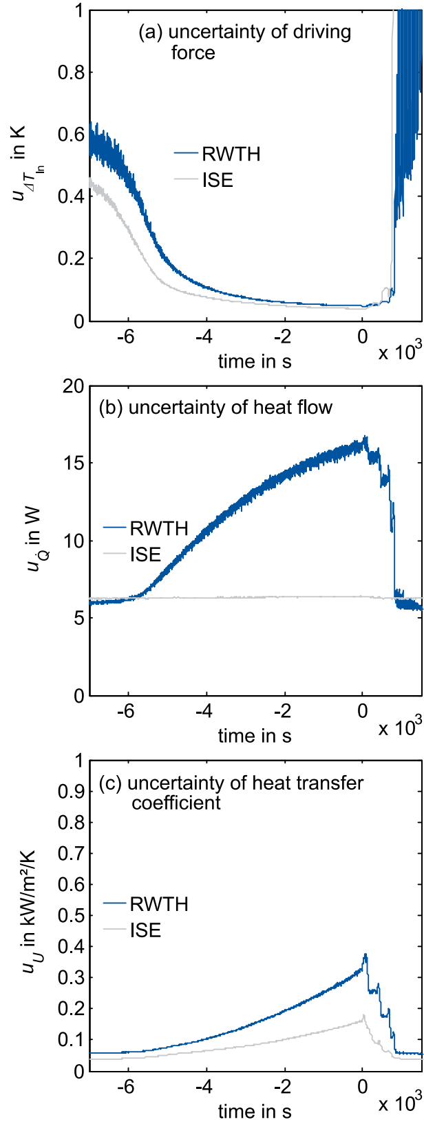
Fig. S111: Uncertainty in measurement for the quantities driving force \Delta T_{in} (a), heat flow \dot{Q} (b) and heat transfer coefficient U (c) shown in Fig. 5 for experiments with parameter set highDF plotted over time. Both experiments (RWTH and ISE) are synchronized at the end of the experiment ( t=0 ) when the first tube loses contact to the refrigerant pool.
