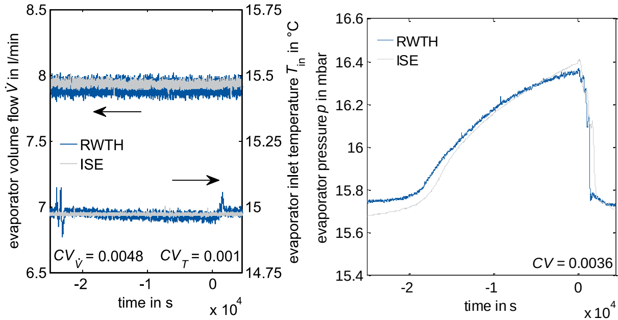
Fig. S17: Operating conditions for experiments with parameter set lowDF plotted over time. Left: evaporator volume flow \dot{V} and inlet temperature T_{in} , right: evaporator pressure p . Both experiments (RWTH and ISE) are synchronized at the end of the experiment ( t=0 ) when the first tube loses contact to the refrigerant pool.
