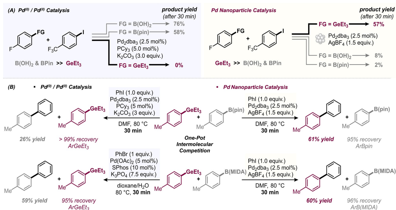
Figure 6. A) Performance of ArGeEt_3 versus established coupling agents in couplings with PhI under Pd^0/Pd^{II} catalysis (left) and nanoparticle catalysis (right). B) Intermolecular competitions in the coupling of PhI with ArGeEt_3 versus ArB(pin) or ArB(MIDA) under Pd^0/Pd^{II} molecular catalysis (left) and nanoparticle catalysis (right). Reaction times: 30 min.
