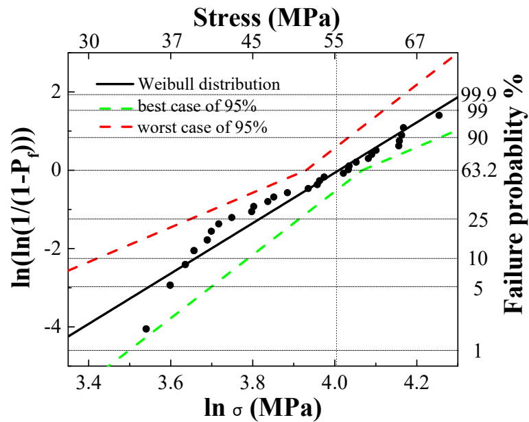
Figure 4.28 Weibull distribution for LLZO.
