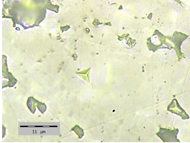
Figure 4.24 Nano-indentation impression in LLZO, load of 100 mN.
