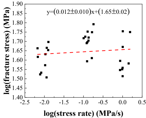
Figure 4.29 Individual fracture stresses of LLZO as a function of loading rates.
