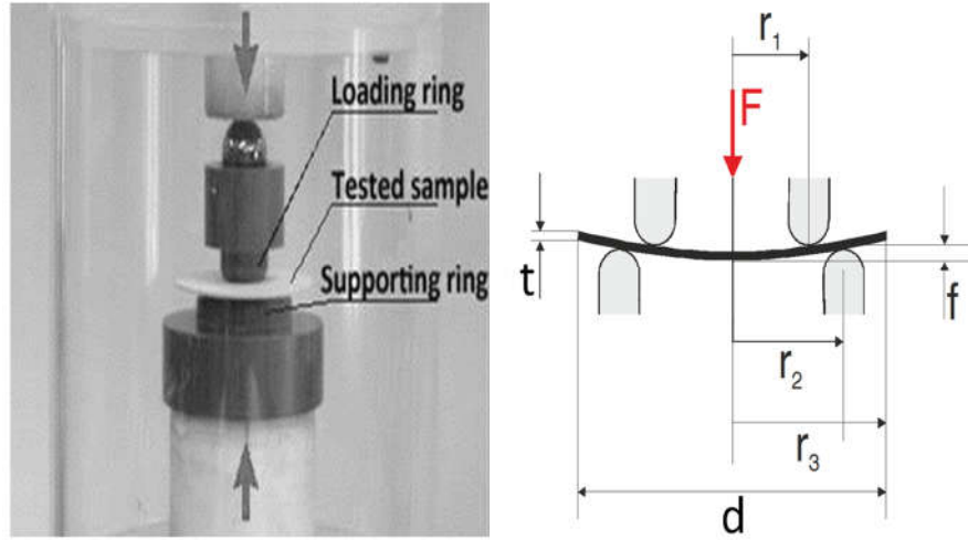
Figure 3.6 The ring-on-ring bending test set-up in IEK-2.
