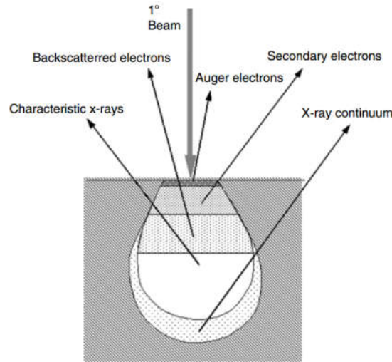
Figure 3.1 Interpretation of the signals produced by the interaction between the electron beam and the sample and the regions from which the signals can be detected [188].
