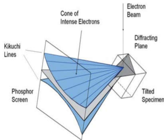
Figure 3.2 Schematic of the intense electrons' cone regarding to the specimen, reflecting plane and phosphor screen [190].
