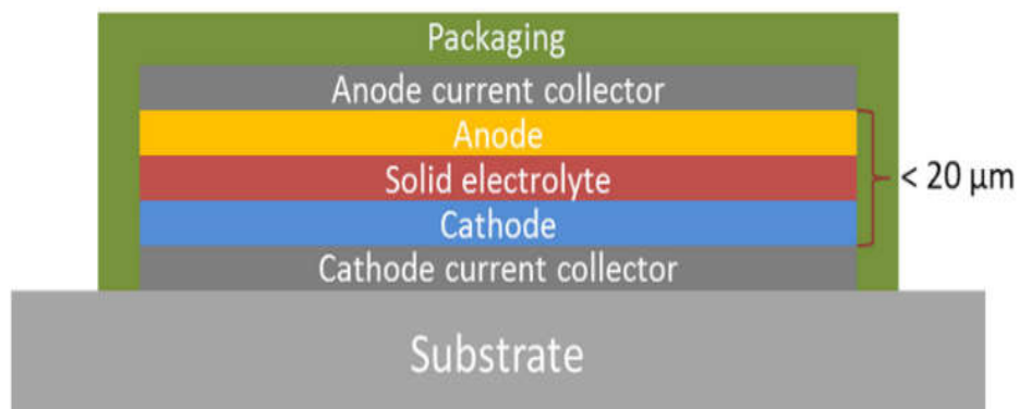
Figure 2.2 Schematic of a planar thin-film micro-battery architecture [9].
