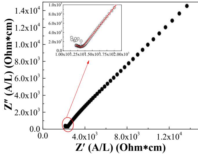
Figure 4.23 Nyquist plot for LLZO at room temperature.
