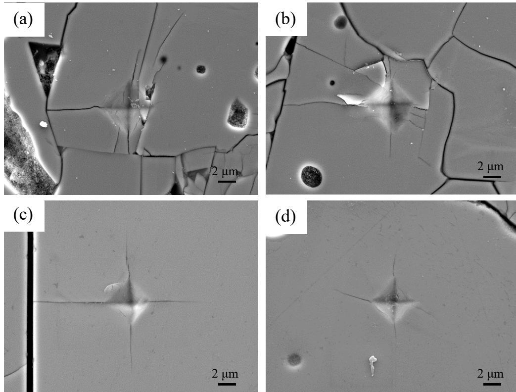
Figure 4.5 Typical SEM images of indents on LATP samples, (a), (b), (c) and (d) represent LATP sintered in 950, 1000, 1050 and 1100 °C, respectively.
