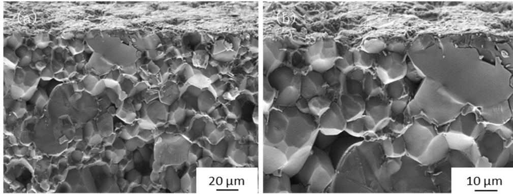
Figure 4.21 SEM fracture cross-section of LLZO.
