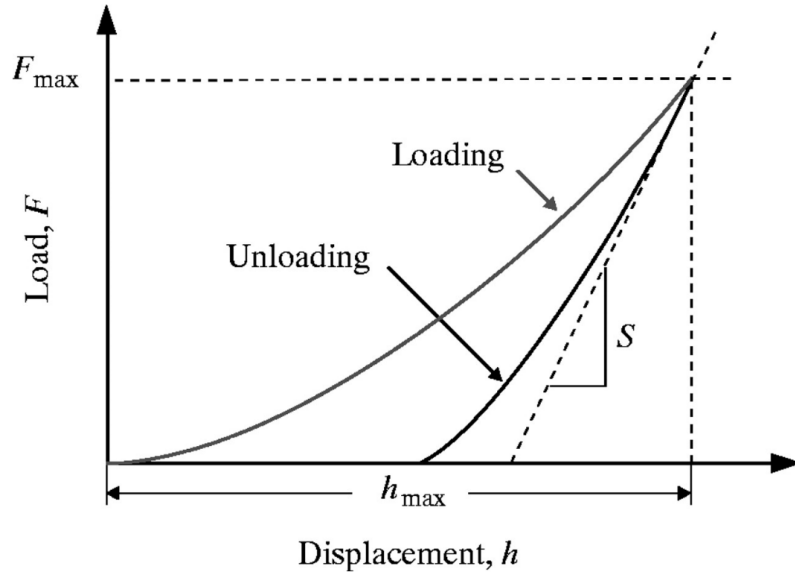
Figure 3.3 Schematic of the load-displacement curve for typical indentation test, in which the S is the contact stiffness.
