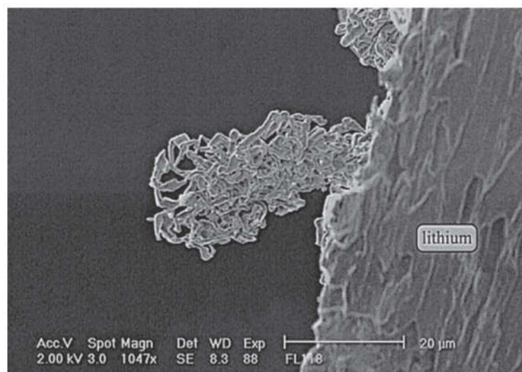
Figure 2.6 Observation of typical lithium dendrites formed on a anode surface [115].
