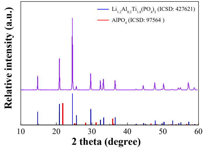
Figure 4.15 XRD pattern of sintered LATP:Si tape.
