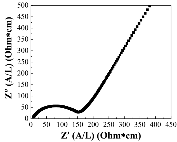
Figure 4.8 Nyquist plot of the LATP material at 25 °C.
