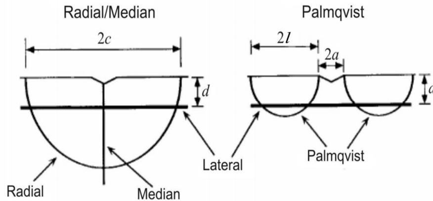
Figure 3.4 Principle scheme of the indentation crack modes [195].
