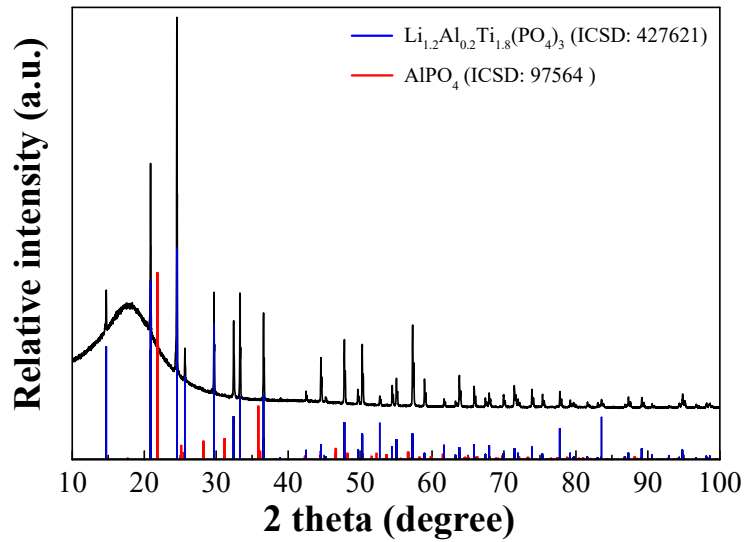
Figure 4.7 XRD pattern of as-sintered LATP sample.
