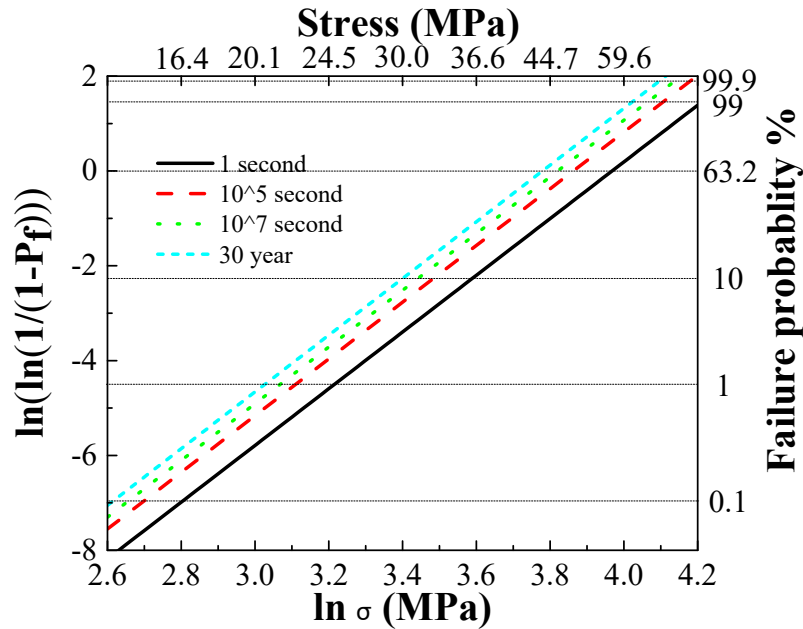
Figure 4.30 Strength-probability-time plots for LLZO.
