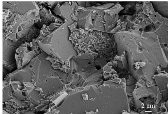
Figure 4.16 SEM micrograph of fracture surface of LATP:Si.
