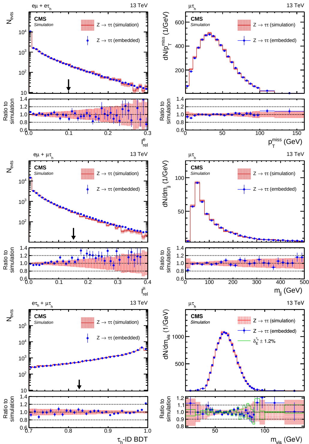
Figure 10. Comparison of \tau -embedded events with a statistically independent sample of simulated Z \rightarrow \tau\tau events. Shown are distributions of (upper left) f_{\text{rel}}^c , (upper right) p_{\text{T}}^{\text{miss}} , (middle left) l_{\text{rel}}^{\mu} , (middle right) m_{\text{jj}} , (lower left) \tau_{\text{h}} -ID BDT, and (lower right) m_{\text{vis}} , as discussed in the text. The black arrows indicate the working points usually used in the target analyses. The blue vertical bars and red-shaded bands correspond to the statistical uncertainty of each sample. The effect of a variation of the \tau_{\text{h}} energy scale of \pm 1.2\% is shown by the green lines.
