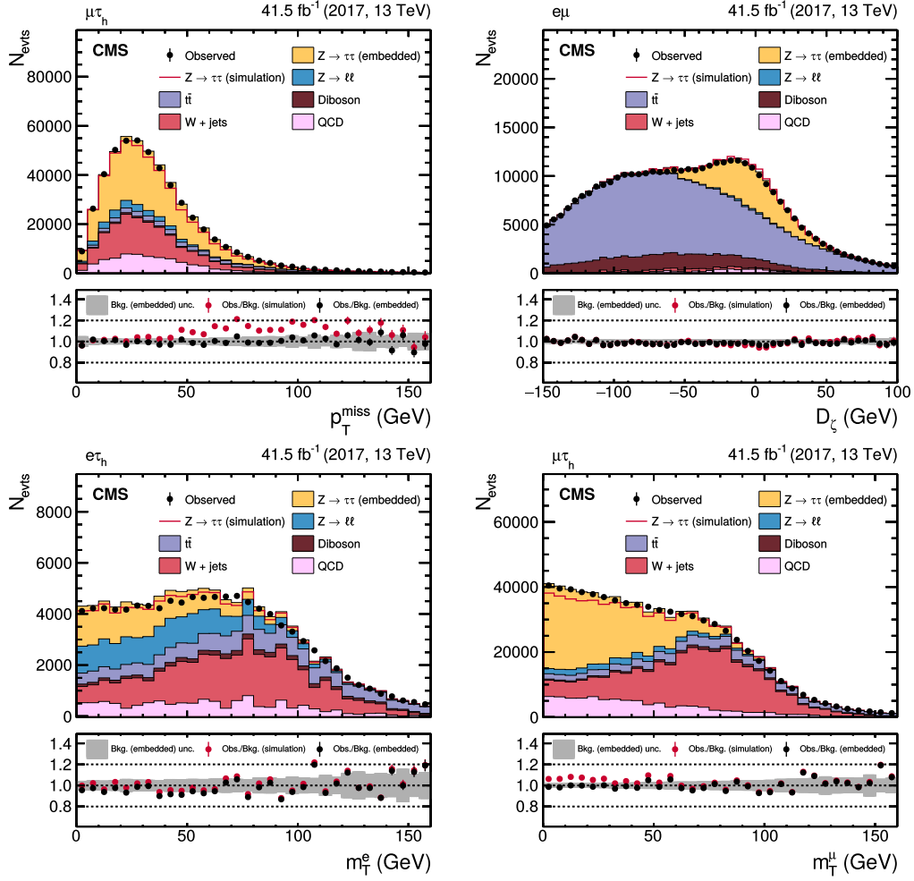
Figure 12. Distributions of (upper left) p_T^{\text{miss}} in the \mu\tau_h final state, (upper right) D_z in the e\mu final state, (lower left) m_T^e in the e\tau_h final state, and (lower right) m_T^\mu in the \mu\tau_h final state. The distributions are shown prior to the maximum likelihood fit described in the text. For these figures, no uncertainties that affect the shape of the distributions have been included in the uncertainty model. The background estimation purely from the CMS simulation is shown as an additional red line.
