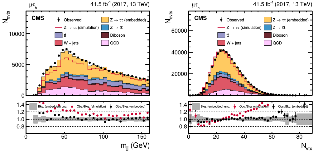
Figure 14. Distributions of (left) m_{jj} and (right) the number of reconstructed primary vertices N_{\text{vtx}} in the \mu\tau_h final state.
