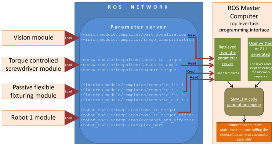
Fig. 11. SMACHA's modular software design supplements the modular hardware design of the robot workcell. Each module within the cell can upload SMACHA templates to the parameter server. This scheme shows an example how the Vision module , the Torque controlled screwdriver module , the Passive flexible fixture module and the Robot 1 module upload their templates to the parameter server. The robot programmer writes a top-level YAML script describing the assembly sequence as a state machine using the templates available on the parameter server. The SMACHA generator then combines these inputs and generates the appropriate computer executable code.
