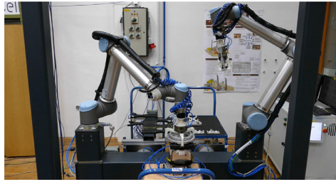
(d) Assembly of a family of airport runway signalling lights.
