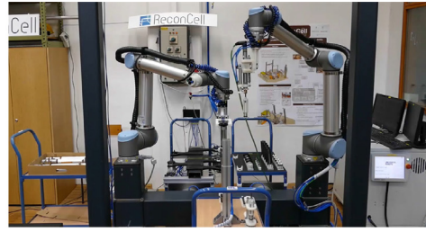
(b) Assembly of a customized linear actuator for smart furniture.
