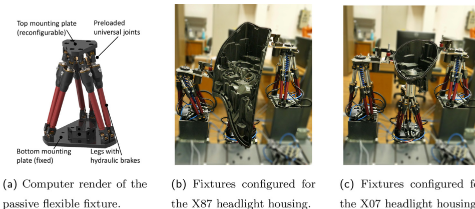
Fig. 4. A passive fixture is designed as a Gough-Stewart platform, containing hydraulic brakes in each leg so that the legs can hold the top platform firmly in the desired position. It is possible to mount various fixturing elements (e. g. centering cones or clamps) on the top platform. To automate the re-positioning of these fixtures, we also installed the male end of the tool exchange system, thus allowing the robot to move the top end of the fixtures when the brakes are released.
