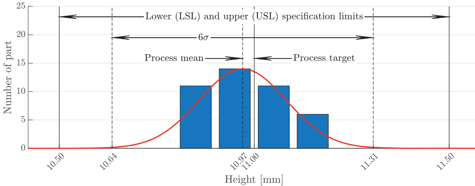
(a) Graphical representation of the heat shield height statistical analysis.
