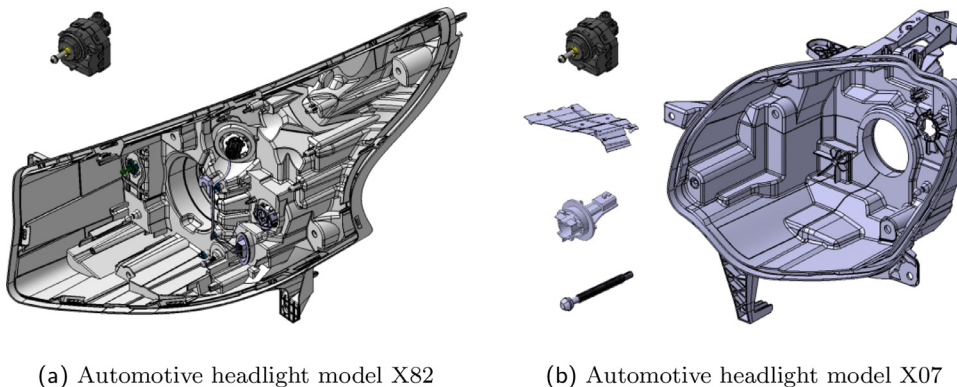
Fig. 15. Two different automotive light housings that were assembled in the proposed workcell and the respective parts that need to be inserted in order to complete the assembly. The left side figure shows the headlight model X82 where only the LWR drive has to be inserted. The right hand figure shows the headlight model X07 with the parts to be inserted (from top to bottom): the LWR drive, a heat shield, a bulb holder and a screw.
