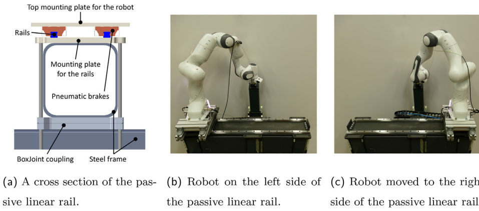
Fig. 3. The developed passive linear rail allows for re-positioning of the robot's base to extend its workspace. The robot is mounted on a platform that can slide along rails and contains pneumatically activated brakes, which disengage before the robot is to be moved. For autonomous re-positioning, the robot attaches itself to the frame with the tool exchange system and then propels its base to the desired new position (Fig. 3b and c). Fig. 3d shows that the arising joint torques are within the limits for all joints.
