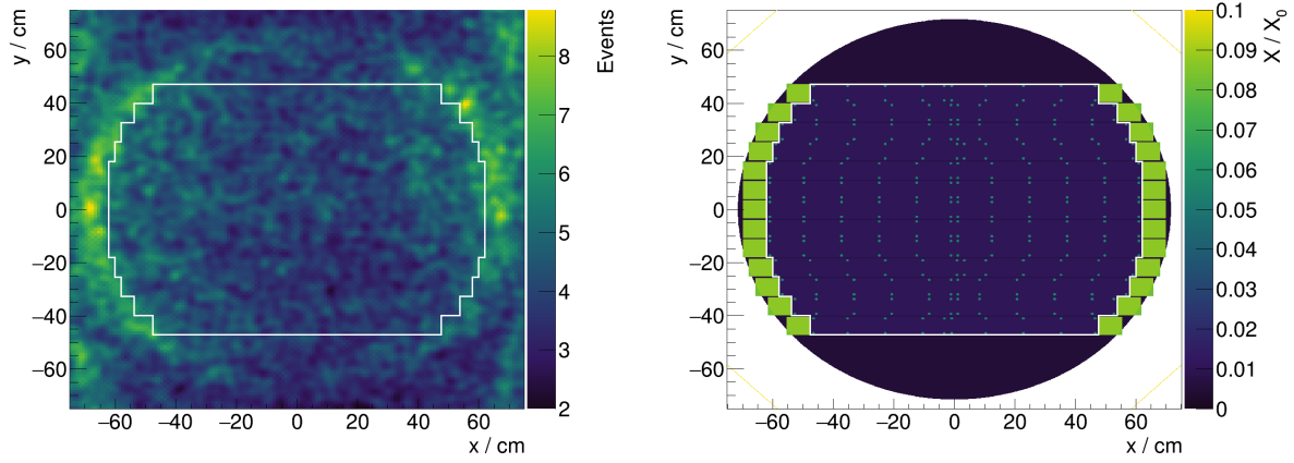
Figure 4.39.: Left: Extrapolation of reconstructed photon directions to the tracker layer 1 plane for events outside of the galactic plane ( |b| > 10^\circ ). Right: Integrated radiation length ( X/X_0 ) in the tracker layer 1 material budget according to the AMS-02 model in the simulation. The white line marks the circumference of the tracker layer 1 active area in both figures.
