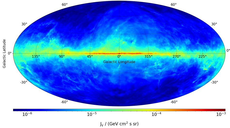
Figure 2.28.: Fermi IEM diffuse \gamma -ray flux at 1 GeV.
