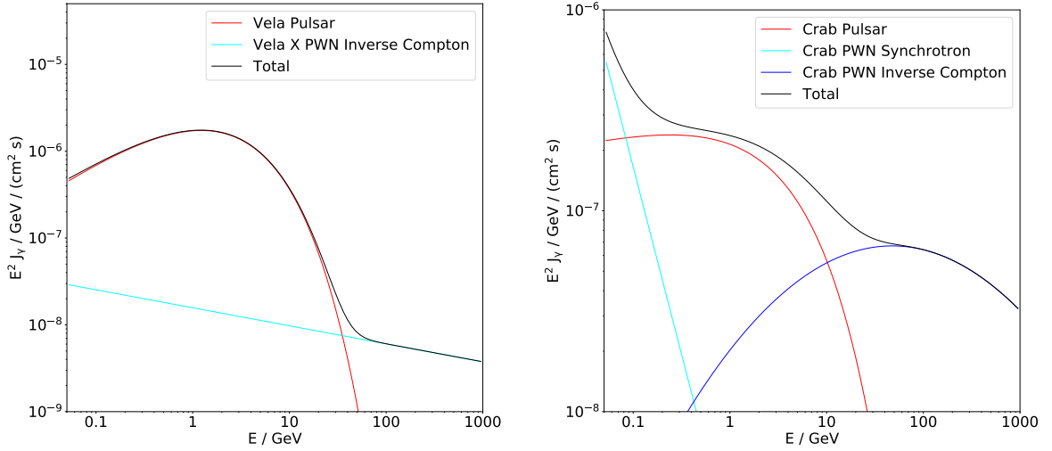
Figure 2.30.: The gamma ray flux of the Vela (left) and Crab (right) pulsars and PWNe, according to the Fermi-LAT 4FGL catalog [109].
