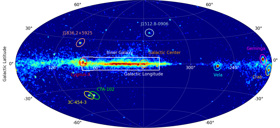
Figure 6.1.: Integrated photon counts in the conversion analysis between 500 MeV and 100 GeV together with the locations of various windows discussed in the text.
