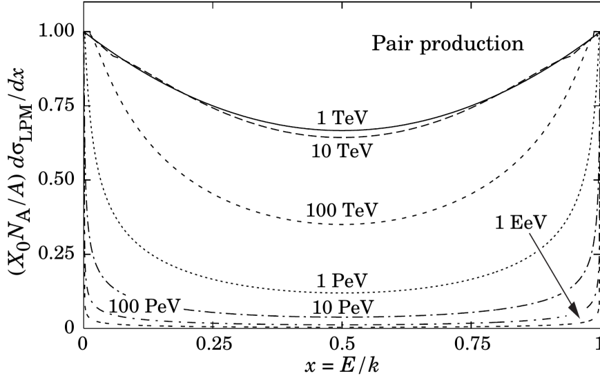
Figure 2.7.: Normalized differential cross section d\sigma/dx for pair production as a function of the fraction electron energy x = E_e/E_\gamma . Figure taken from the Particle Data Group's Review of Particle Physics [54].
