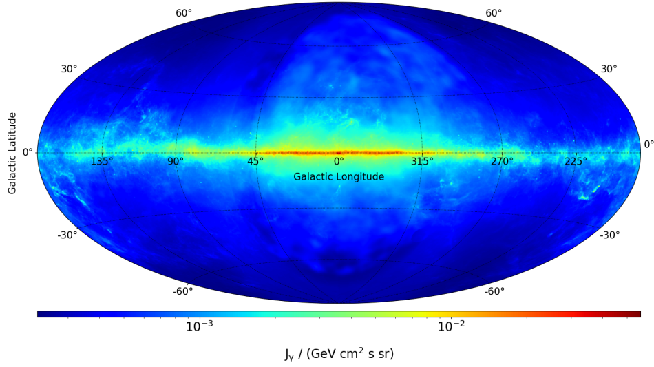
Figure 2.27.: Fermi IEM diffuse \gamma -ray flux at 50 MeV.
