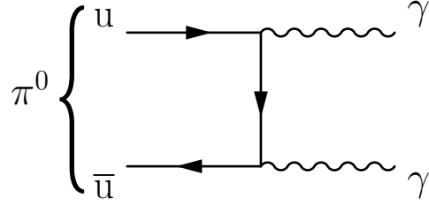
Figure 2.1.: Leading order Feynman diagram for the decay of \pi^0 mesons into two photons.
