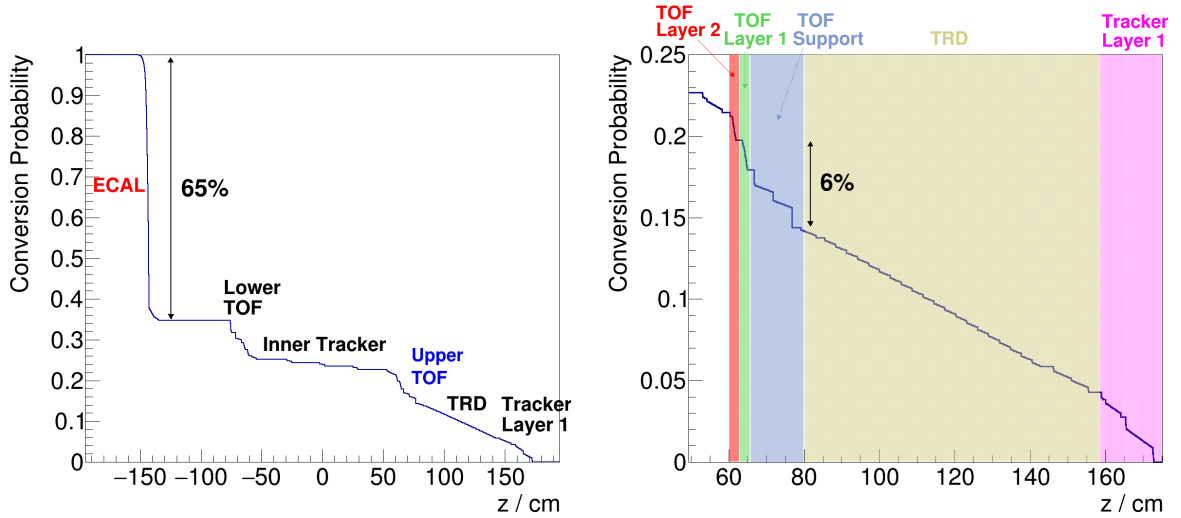
Figure 4.3.: Integrated probability for photon conversions, based on the \frac{x}{X_0} distribution in the Monte-Carlo simulation for a perpendicular trajectory passing through x = y = 5 cm. Left: Entire detector, Right: Zoom into the upper detector region.
