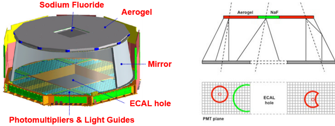
Figure 3.26.: Left: Overview of the components of the RICH detector [166]. Right: Illustration of the various forms of Cherenkov rings, depending on where the particle passes through the radiator.
