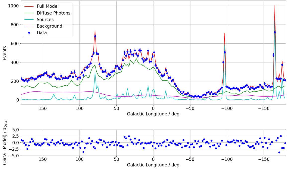
Figure 4.44.: One dimensional comparison of measured photon counts between 500 MeV and 100 GeV in the galactic plane ( |b| < 8^\circ ) for the vertex analysis with the model prediction including the background component as a function of galactic longitude. The lower panel shows the pull distribution, uncertainties are statistical only.
