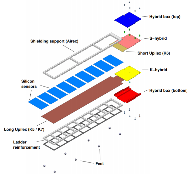
Figure 3.13.: Schematic view of the components of a tracker silicon ladder [158].
