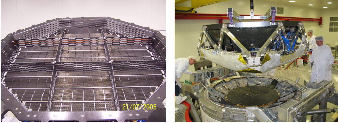
Figure 3.19.: Left: The partially assembled transition radiation detector [164]. The fleece radiator above the visible layer of tubes, as well as the four uppermost layers have yet to be installed. Right: The installation of the TRD on top of AMS [164].
