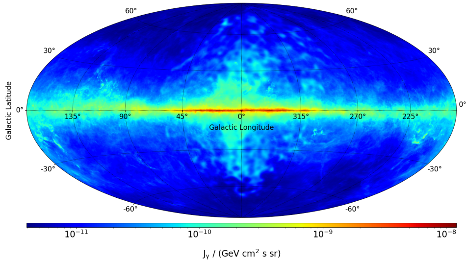
Figure 2.29.: Fermi IEM diffuse \gamma -ray flux at 100 GeV.
