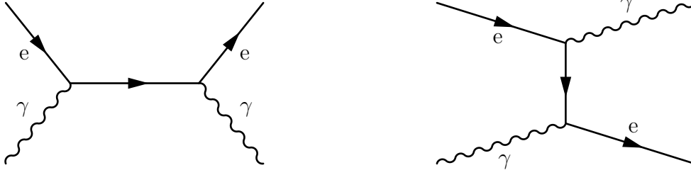
Figure 2.5.: Leading order Feynman diagrams for (inverse) Compton scattering. Left: s-channel, Right: t-channel.
