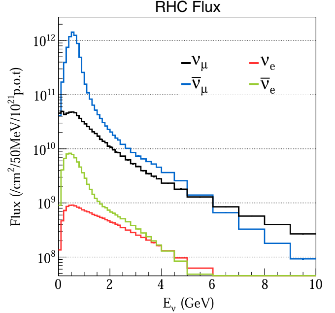
FIG. 1. The RHC flux given per \text{cm}^2/50 \text{ MeV}/10^{21} \text{ PoT} as a function of energy at the ND280 detector for the different neutrino components ( \bar{\nu}_\mu , \nu_\mu , \bar{\nu}_e , \nu_e ).
