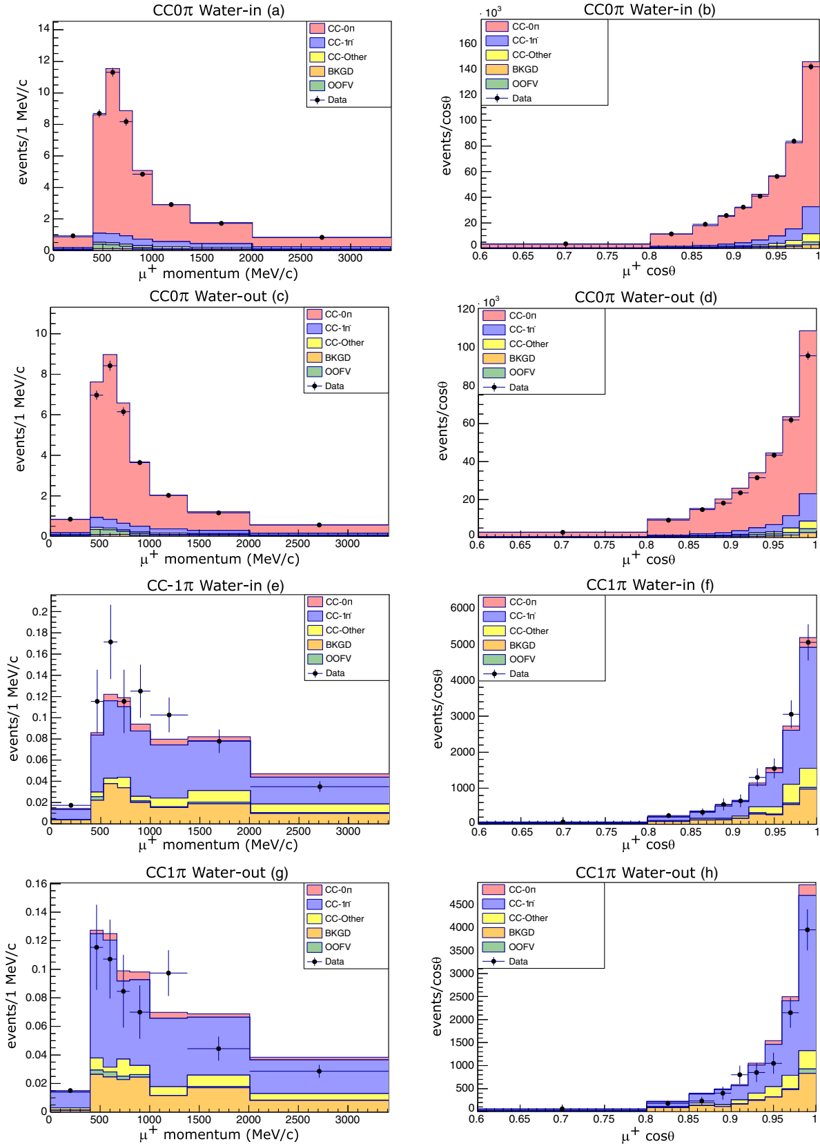
FIG. 3. Comparisons of lab-frame momentum (left column) and \cos\theta (right column) distributions between data (black dots with error bars) and NEUT simulation predictions before fitting (stacked color bands). The CC-0 \pi selections have been applied on the water-in samples [(a) and (b)] and water-out samples [(c) and (d)]. The CC-1 \pi selections have been applied on the water-in samples [(e) and (f)] and water-out samples [(g) and (h)].
