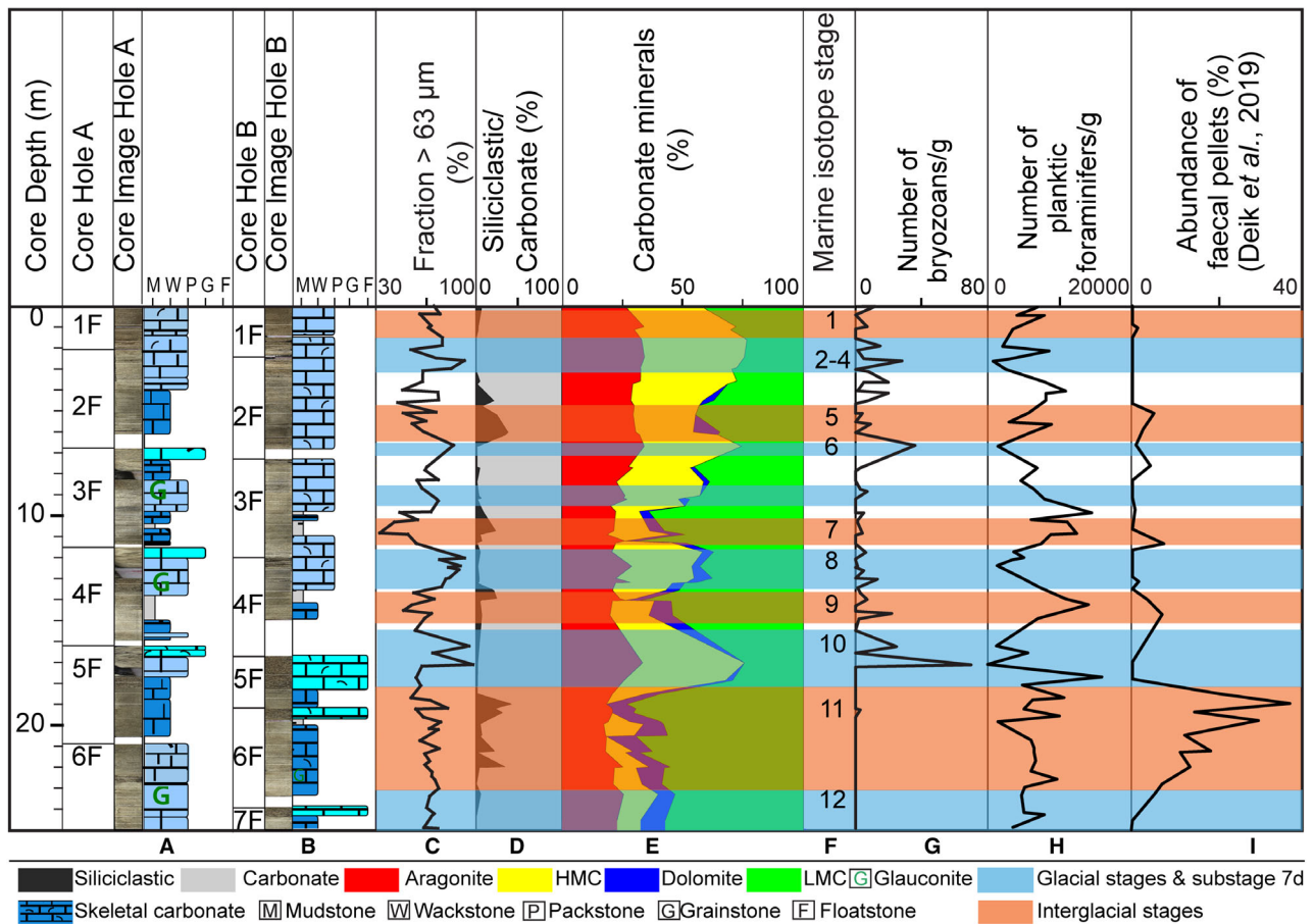
Fig. 3. Lithostratigraphic summary for Integrated Ocean Drilling Program (IODP) Hole U1460A (A) and IODP Hole U1460B (B) (Gallagher et al. , 2017). (C) Grain-size fraction >63 µm of sediments from holes A and B (Courtillat, 2019). (D) Siliciclastic (black) versus carbonate (grey) content. (E) Carbonate mineralogy (aragonite, red; high-Mg calcite, yellow; dolomite, blue; low-Mg calcite, green). (F) Integrated stratigraphy based on a comparison between the two alternative age models shown in Fig. 2. (G) Abundance of bryozoans in one gram of sediment. (H) Abundance of planktic foraminifera in one gram of sediment. (I) Relative abundance of faecal pellets in the fine to medium sand-sized (125 to 500 µm) sediment fraction (Deik et al. , 2019).
