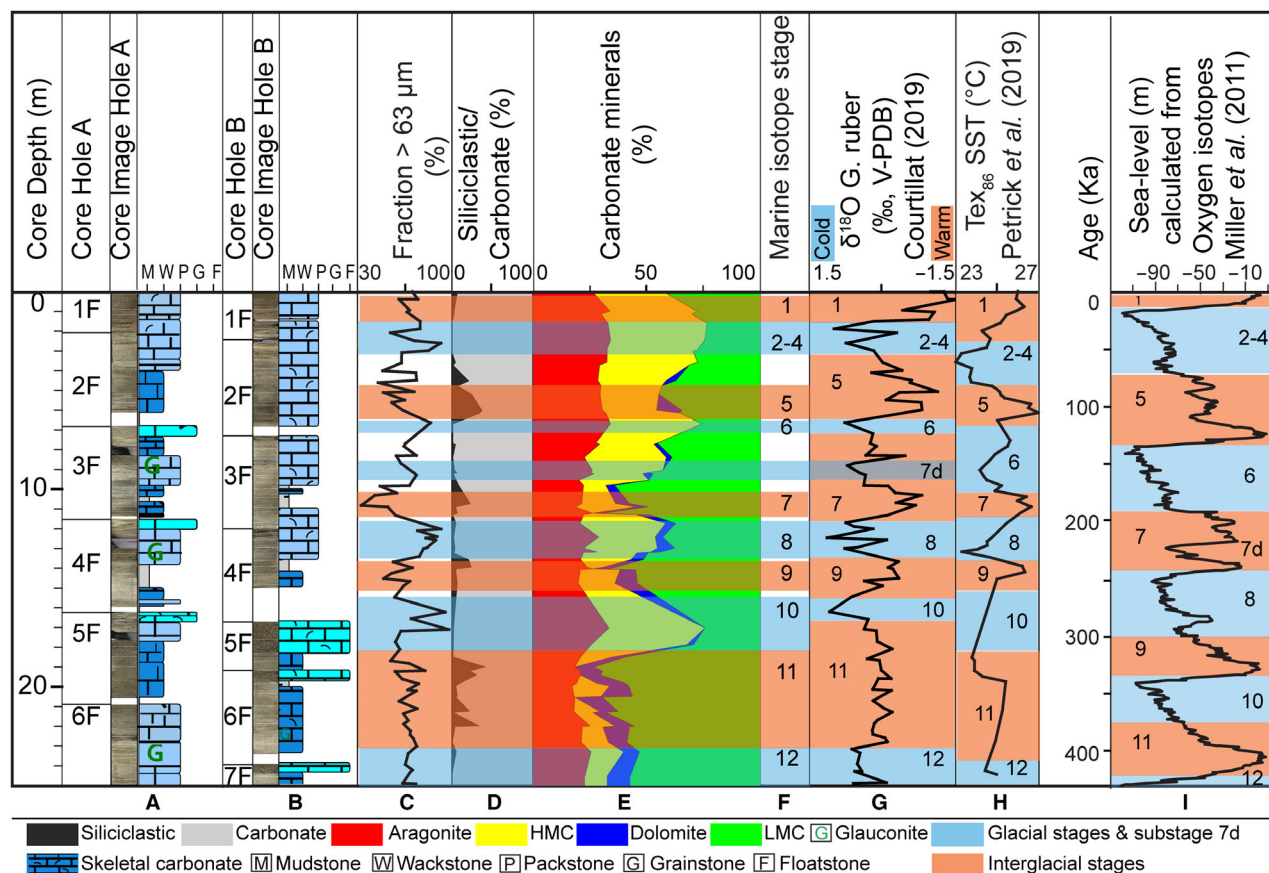
Fig. 2. Lithostratigraphic summary for Integrated Ocean Drilling Program (IODP) Hole U1460A (A) and IODP Hole U1460B (B) (Gallagher et al. , 2017). (C) Grain-size fraction >63 µm of sediments from holes A and B (Courtillat, 2019). (D) Siliciclastic (black) versus carbonate (grey) content. (E) Carbonate mineralogy (aragonite, red; high-Mg calcite, yellow; dolomite, blue; low-Mg calcite, green). (F) Integrated stratigraphy based on a comparison between the two alternative age models shown in (G) and (H). (G) Age model from Courtillat (2019) based on \delta^{18}\text{O} Globigerinoides ruber (shown), ^{14}\text{C} ages and G. menardii complex abundance data. (H) Age model from Petrick et al. (2019) derived from tuning of the TEX 86 temperatures to the benthic isotope stack LR04. (I) Sea-level curve calculated from oxygen isotopes (Miller et al. , 2011). Note: The time axis applies only for (I).
