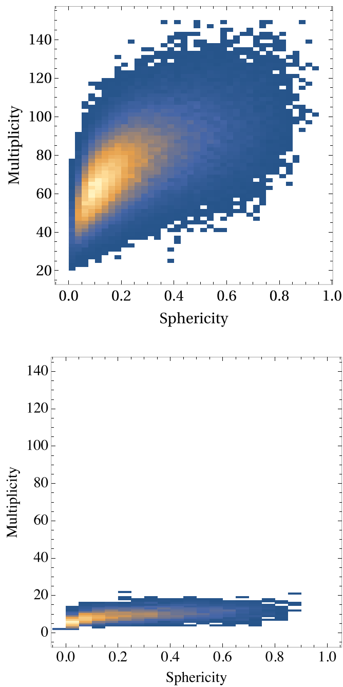
Figure 92. Correlation between sphericity and hadron multiplicity for events generated with parton shower (top) and AdS/CFT-inspired models with boundary interaction (bottom).
