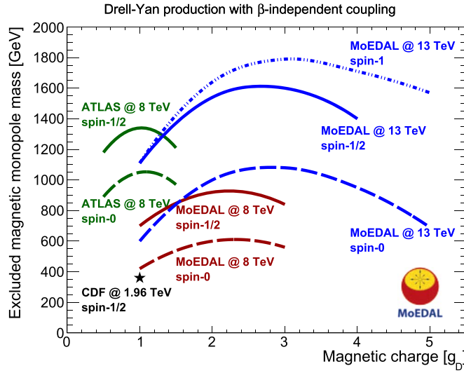
Figure 58. Magnetic monopole mass limits from CDF [429], ATLAS [215] and MoEDAL searches [311, 422] as a function of magnetic charge for various spins, assuming a Drell–Yan pair-production mechanism.
