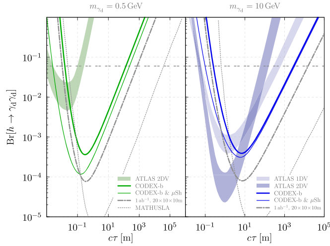
Figure 68. Comparison of experimental sensitivity to the BSM decay of an SM-like Higgs to dark photons with and without the muon shadow (' \mu\text{Sh} ') for a few different existing and proposed detectors. The \gamma_d \rightarrow \mu\mu branching ratio is taken from e^+e^- data [458]. The CODEX-b sensitivity here is the so-called 'optimistic' reach, with \mathcal{L} = 1 \text{ ab}^{-1} and a larger volume, assuming DELPHI is removed. From [104].
