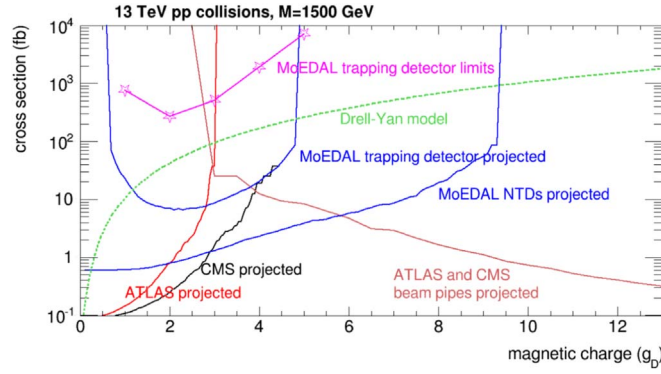
Figure 9. Comparison of the MoEDAL, ATLAS and CMS reaches for magnetic monopoles. The curves assume three signal events and a total integrated luminosity of 50 \text{ fb}^{-1} for 13 TeV collisions. Updated version of existing figure in [310]. Note that the CMS curve relies on the expected performance of their detector.
