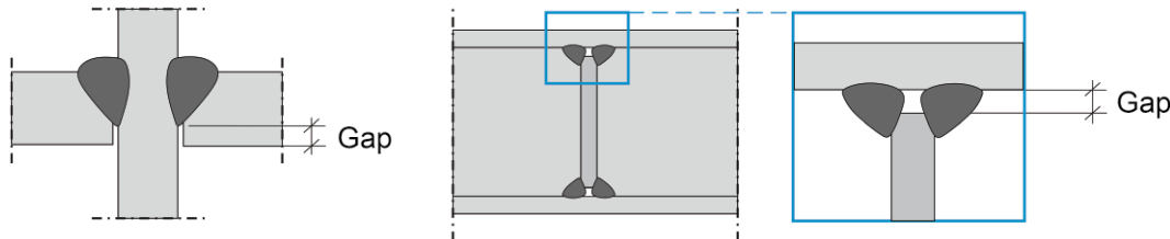
Fig. 15 Gaps in cruciform joints and stiffened beams
