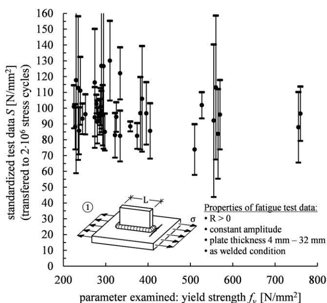
Fig. 4 Standardized scatter bands with 5% and 95% survival probability as a function of the yield stress for test data on longitudinal attachment (test data normalized to 2 million cycles)
