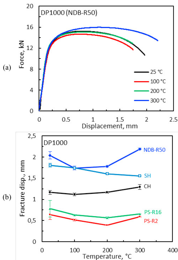
Fig. 5. (a) The force–displacement curves of the NDB-R50 samples of DP1000 at different temperatures; (b) the fracture displacement of various geometries of the DP1000 at different temperatures.
