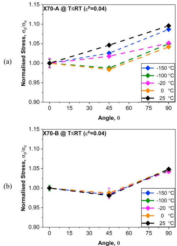
Fig. 3. The stress directionality of the X70-A (a) and X70-B (b) at the plastic strain of 0.04 at different deformation temperatures.
