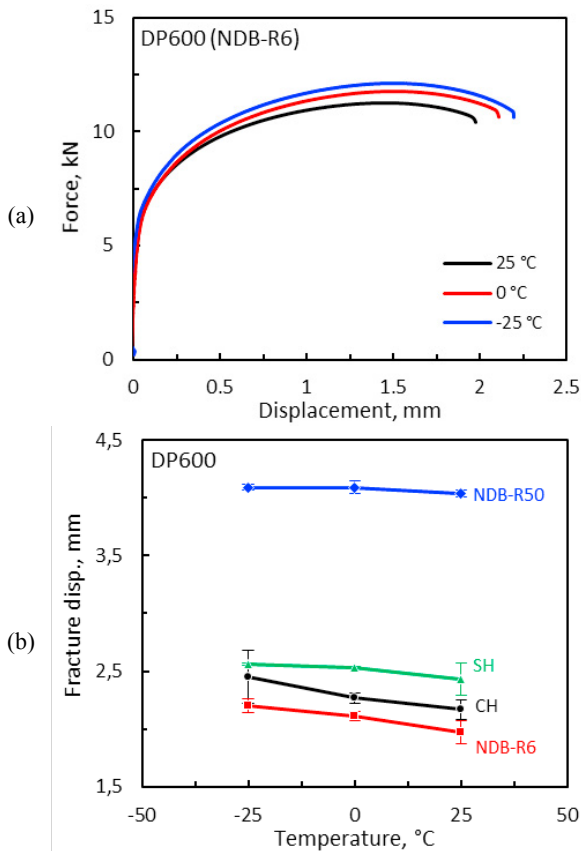
Fig. 7. ((a) The force–displacement curves of the NDB-R6 samples of DP600 at different temperatures; (b) the fracture displacement of various geometries of the DP600 at different temperatures.
