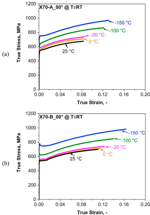
Fig. 2. The true stress–strain curves of X70-A (a) and X70-B (b) along the rolling direction under different deformation temperatures from room temperature to -150\text{ }^{\circ}\text{C} .
