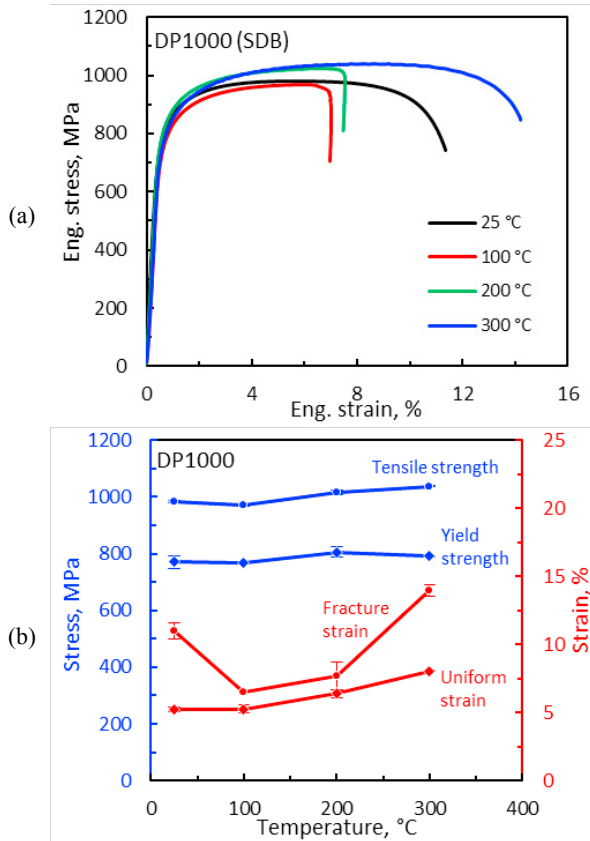
Fig. 4. (a) The engineering stress–strain curves of DP1000 along the rolling direction at different temperatures; (b) the temperature dependence of the main tensile properties.
