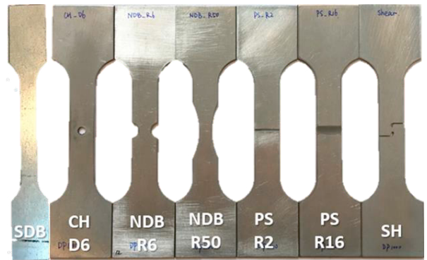
Fig. 1. The sample geometries for the testing program. (Adapted from Liu, et al. [14]).
