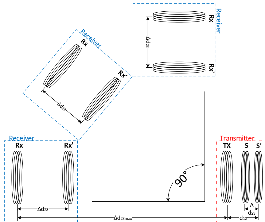
Figure 13. Positioning of receiver for the measurement of angle efficiency.
