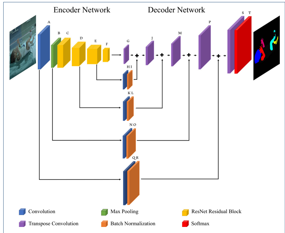
Fig. 2 Proposed encoder-decoder structure based on the architecture proposed by Olivera et al. [21] with a modified version of the ResNet-50 [26] as encoder. Rectified linear units (ReLUs) are omitted for reasons of brevity
