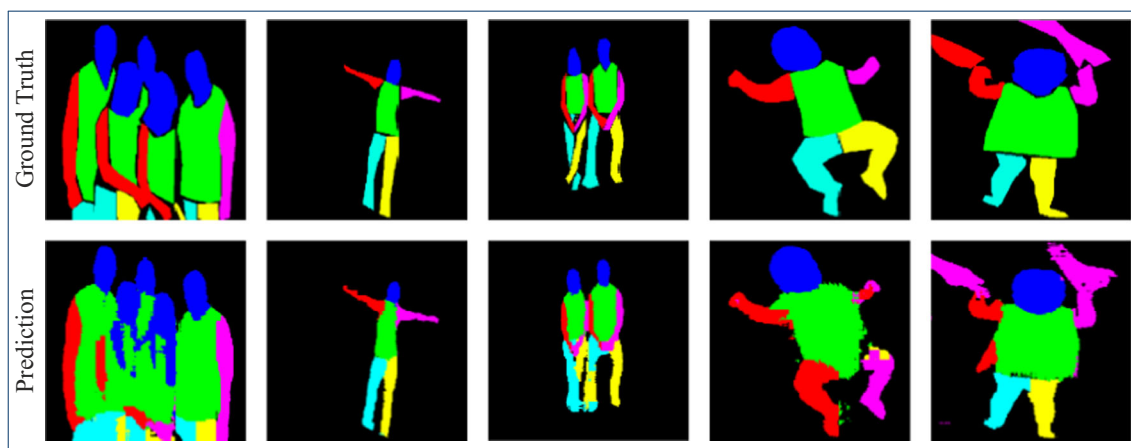
Fig. 5 Qualitative results of the proposed “batchnorm” model on the PASCAL human parts and Freiburg sitting people dataset
