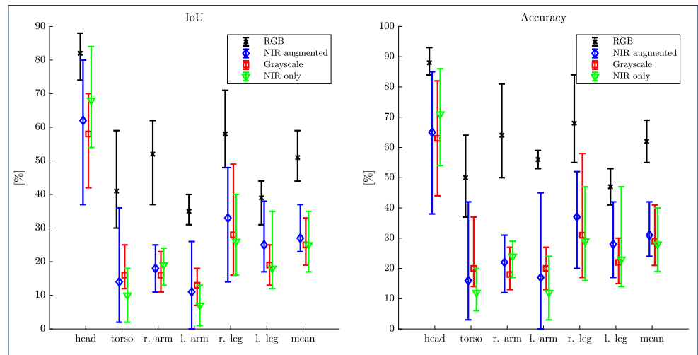
Fig. 6 Quantitative results of the proposed CNN model “batchnorm” on the NICU dataset for the 5-folds. The training and validation images are downsampled by a factor of two in both dimensions (i.e., 960 \times 576 ) using bilinear interpolation. The bars show minimum, mean, and maximum value
