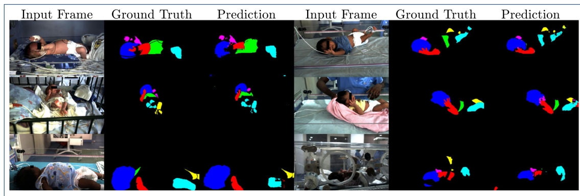
Fig. 7 Qualitative segmentation results for the RGB data. Images were individually optimized (brightens, contrast, white balance) for visualization purposes. Note that the caregivers’ hands are ignored by the algorithm
