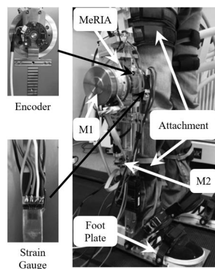
Figure 1: Setup of the unilateral lower limb exoskeleton with the MeRIA on a treadmill.
